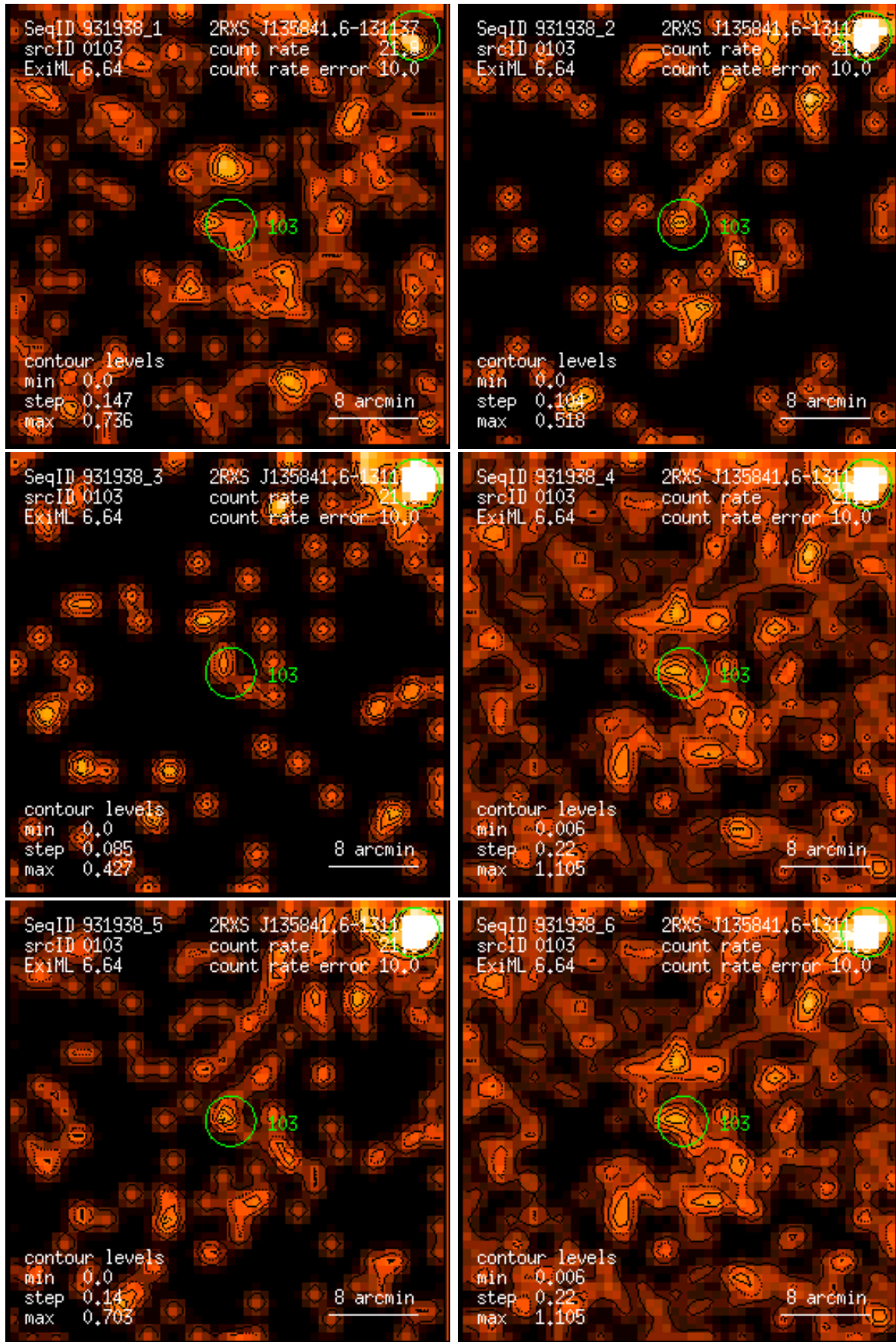
Figure 103: RASS 931938: detection 0103: band rate images, Gaussian filter: (1) PSPC channels 11 – 41, (2) 52 – 90, (3) 91 – 201, (4) 11 – 235, (5) 52 – 201, (6) 11 – 201. Broad band rates in counts/ks. Band rate contour levels in counts/ks/arcmin 2 .
