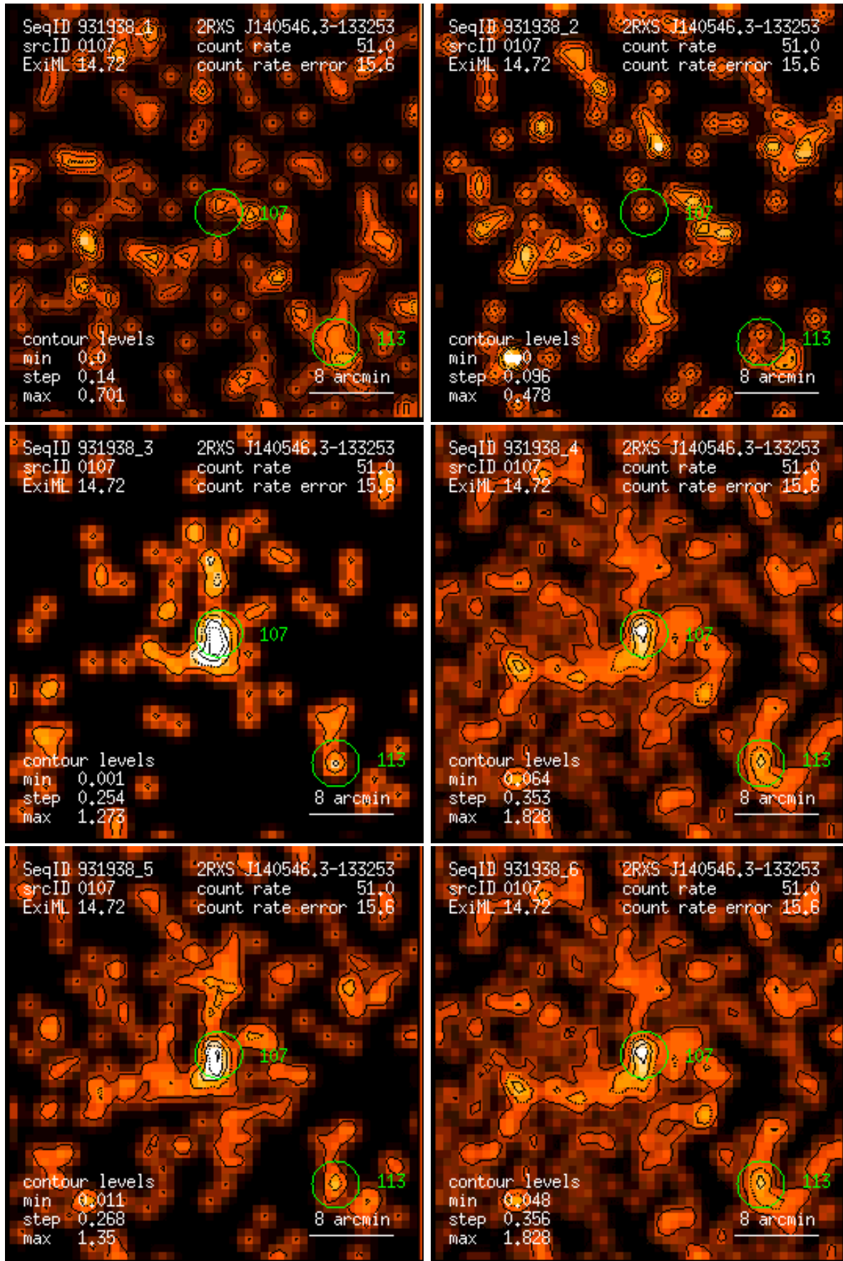
Figure 107: RASS 931938: detection 0107: band rate images, Gaussian filter: (1) PSPC channels 11 – 41, (2) 52 – 90, (3) 91 – 201, (4) 11 – 235, (5) 52 – 201, (6) 11 – 201. Broad band rates in counts/ks. Band rate contour levels in counts/ks/arcmin 2 .
