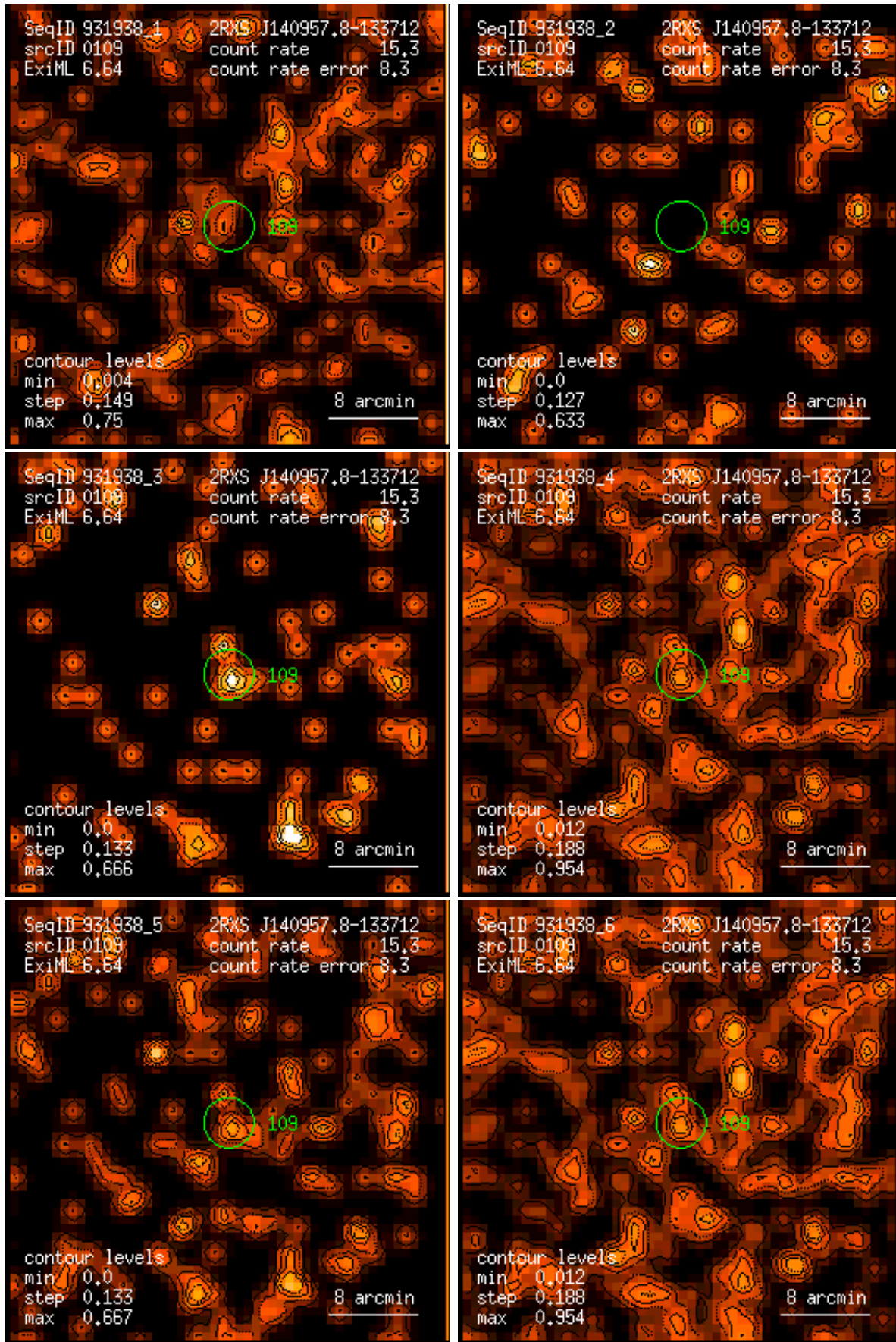
Figure 109: RASS 931938: detection 0109: band rate images, Gaussian filter: (1) PSPC channels 11 – 41, (2) 52 – 90, (3) 91 – 201, (4) 11 – 235, (5) 52 – 201, (6) 11 – 201. Broad band rates in counts/ks. Band rate contour levels in counts/ks/arcmin 2 .
