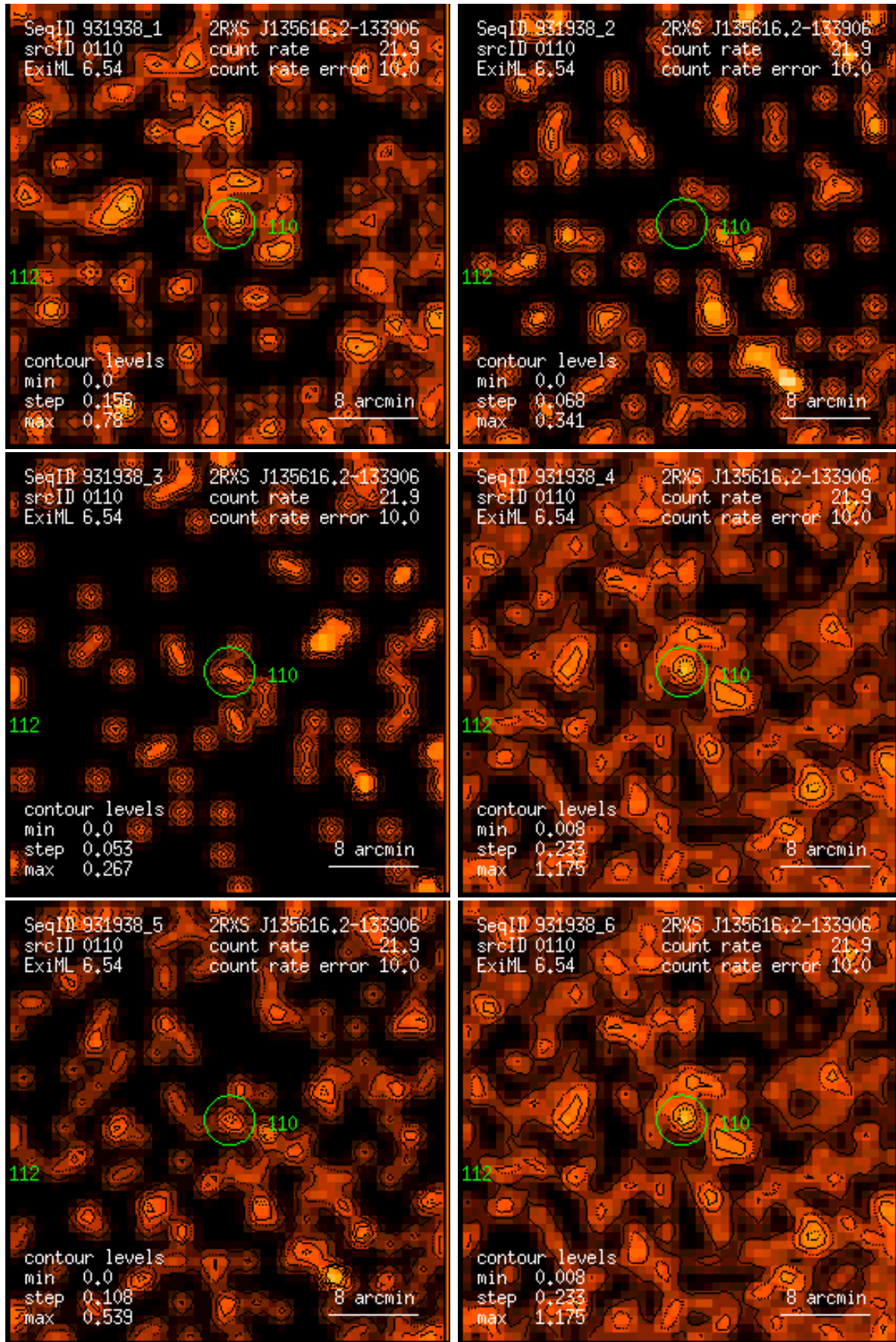
Figure 110: RASS 931938: detection 0110: band rate images, Gaussian filter: (1) PSPC channels 11 – 41, (2) 52 – 90, (3) 91 – 201, (4) 11 – 235, (5) 52 – 201, (6) 11 – 201. Broad band rates in counts/ks. Band rate contour levels in counts/ks/arcmin 2 .
