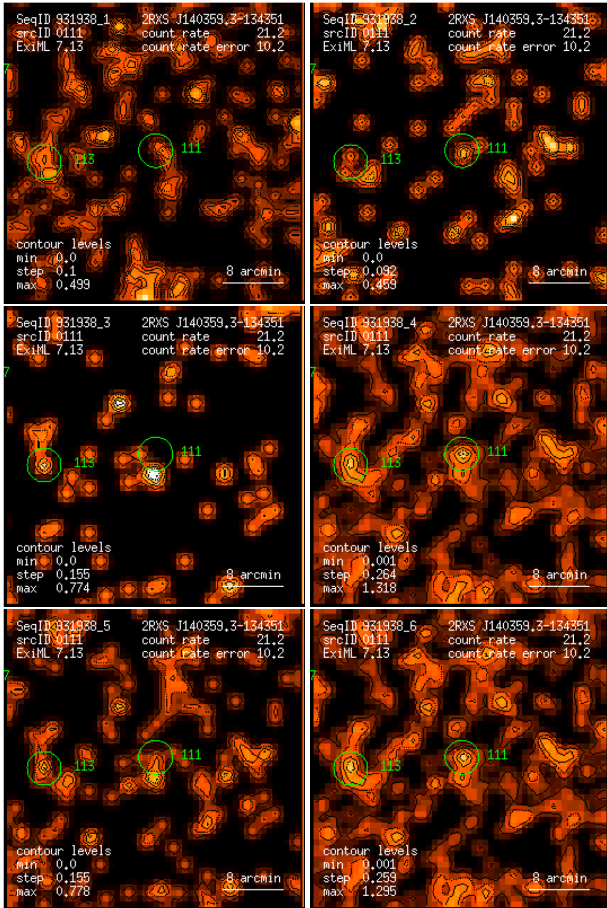
Figure 111: RASS 931938: detection 0111: band rate images, Gaussian filter: (1) PSPC channels 11 – 41, (2) 52 – 90, (3) 91 – 201, (4) 11 – 235, (5) 52 – 201, (6) 11 – 201. Broad band rates in counts/ks. Band rate contour levels in counts/ks/arcmin 2 .
