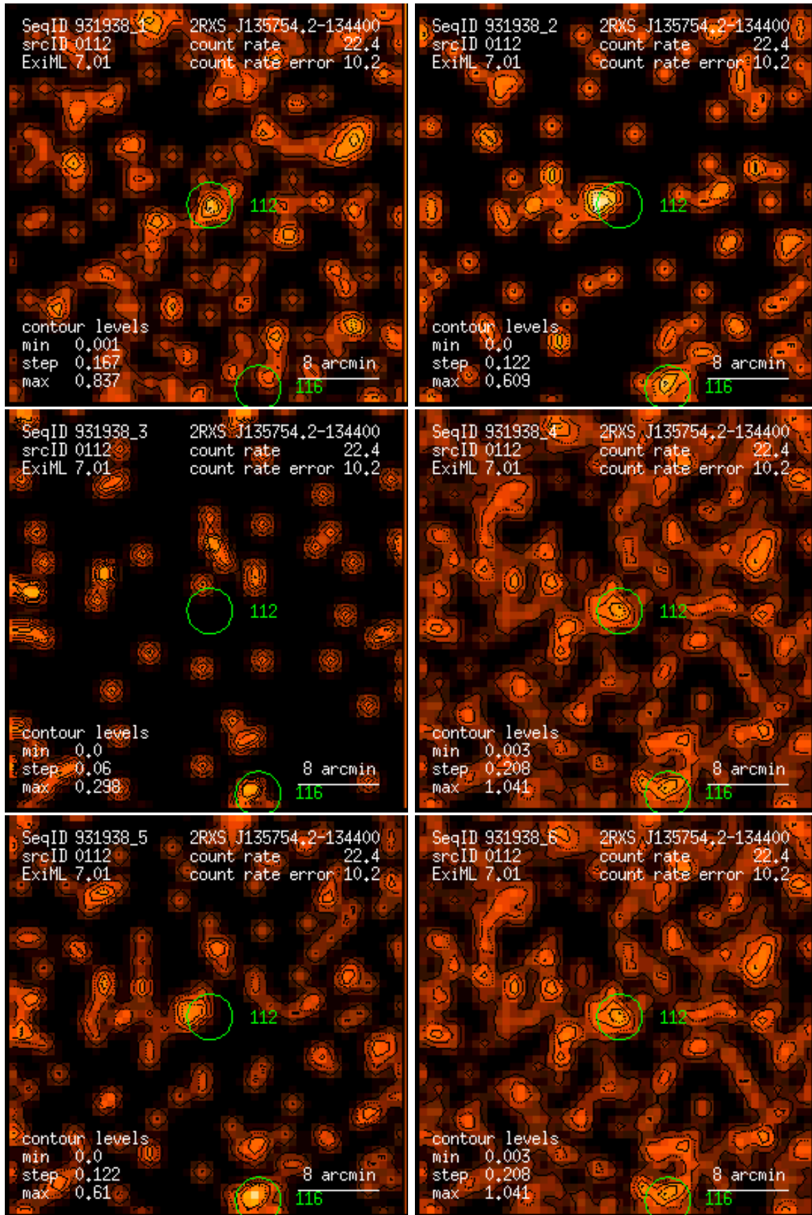
Figure 112: RASS 931938: detection 0112: band rate images, Gaussian filter: (1) PSPC channels 11 – 41, (2) 52 – 90, (3) 91 – 201, (4) 11 – 235, (5) 52 – 201, (6) 11 – 201. Broad band rates in counts/ks. Band rate contour levels in counts/ks/arcmin 2 .
