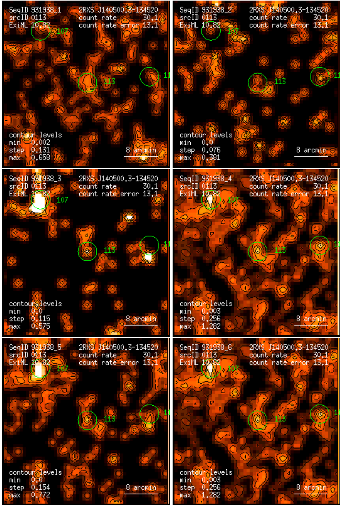
Figure 113: RASS 931938: detection 0113: band rate images, Gaussian filter: (1) PSPC channels 11 – 41, (2) 52 – 90, (3) 91 – 201, (4) 11 – 235, (5) 52 – 201, (6) 11 – 201. Broad band rates in counts/ks. Band rate contour levels in counts/ks/arcmin 2 .
