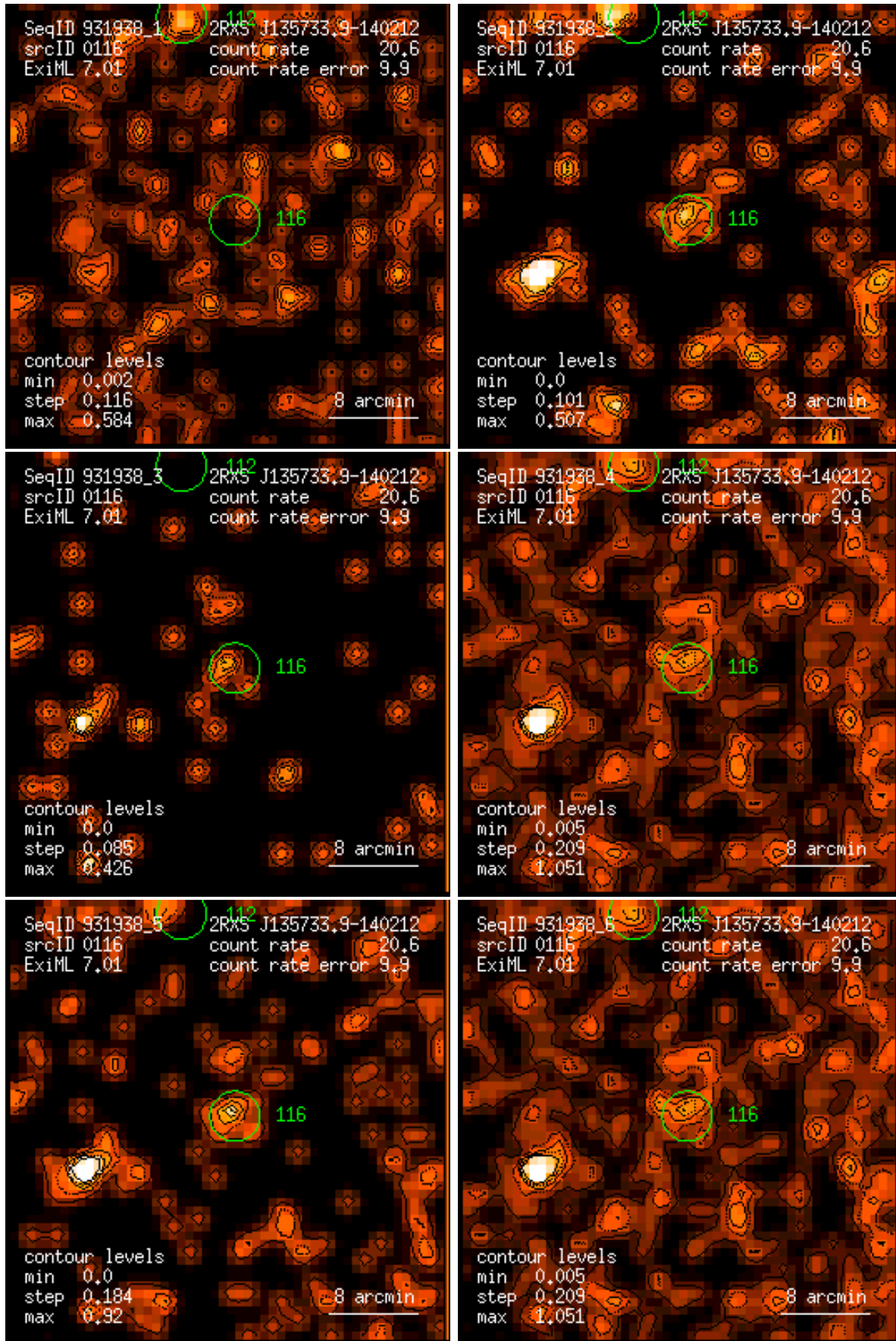
Figure 116: RASS 931938: detection 0116: band rate images, Gaussian filter: (1) PSPC channels 11 – 41, (2) 52 – 90, (3) 91 – 201, (4) 11 – 235, (5) 52 – 201, (6) 11 – 201. Broad band rates in counts/ks. Band rate contour levels in counts/ks/arcmin 2 .
