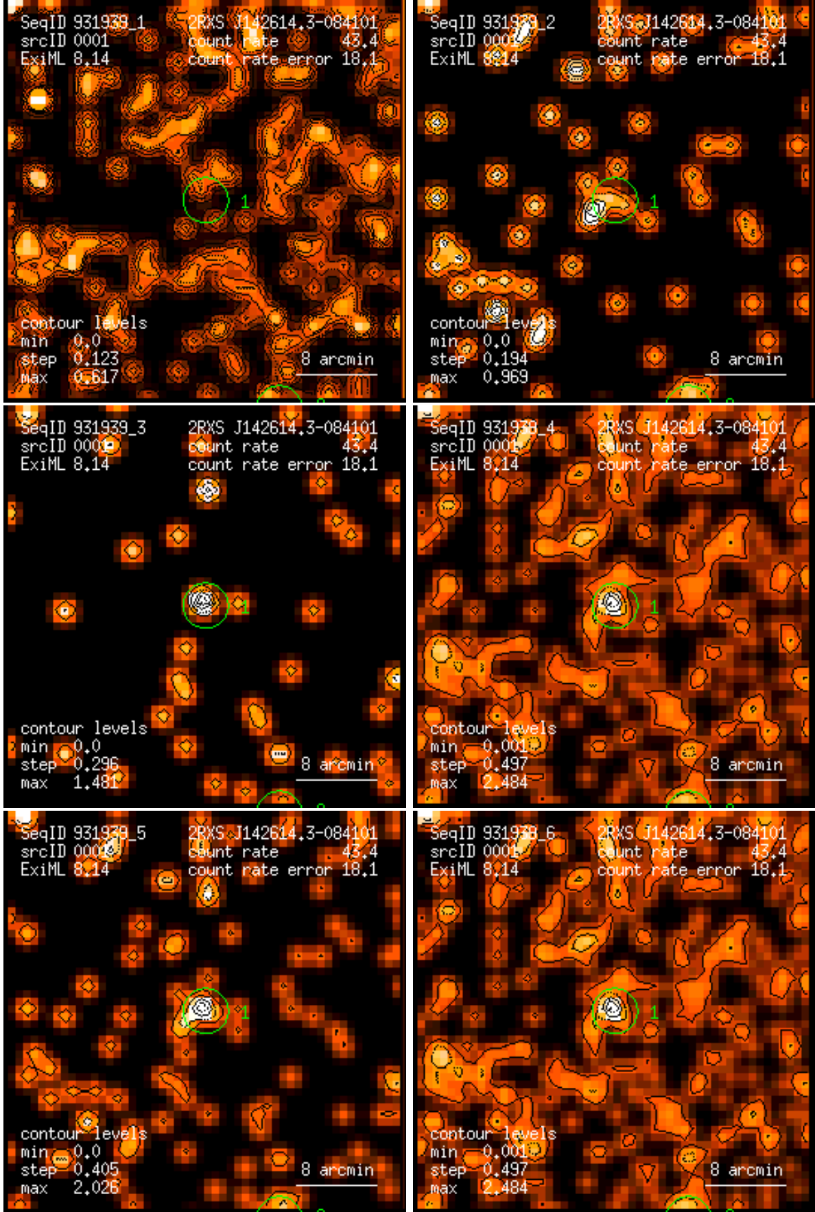
Figure 1: RASS 931939: detection 0001: band rate images, Gaussian filter: (1) PSPC channels 11 – 41, (2) 52 – 90, (3) 91 – 201, (4) 11 – 235, (5) 52 – 201, (6) 11 – 201. Broad band rates in counts/ks. Band rate contour levels in counts/ks/arcmin 2 .
