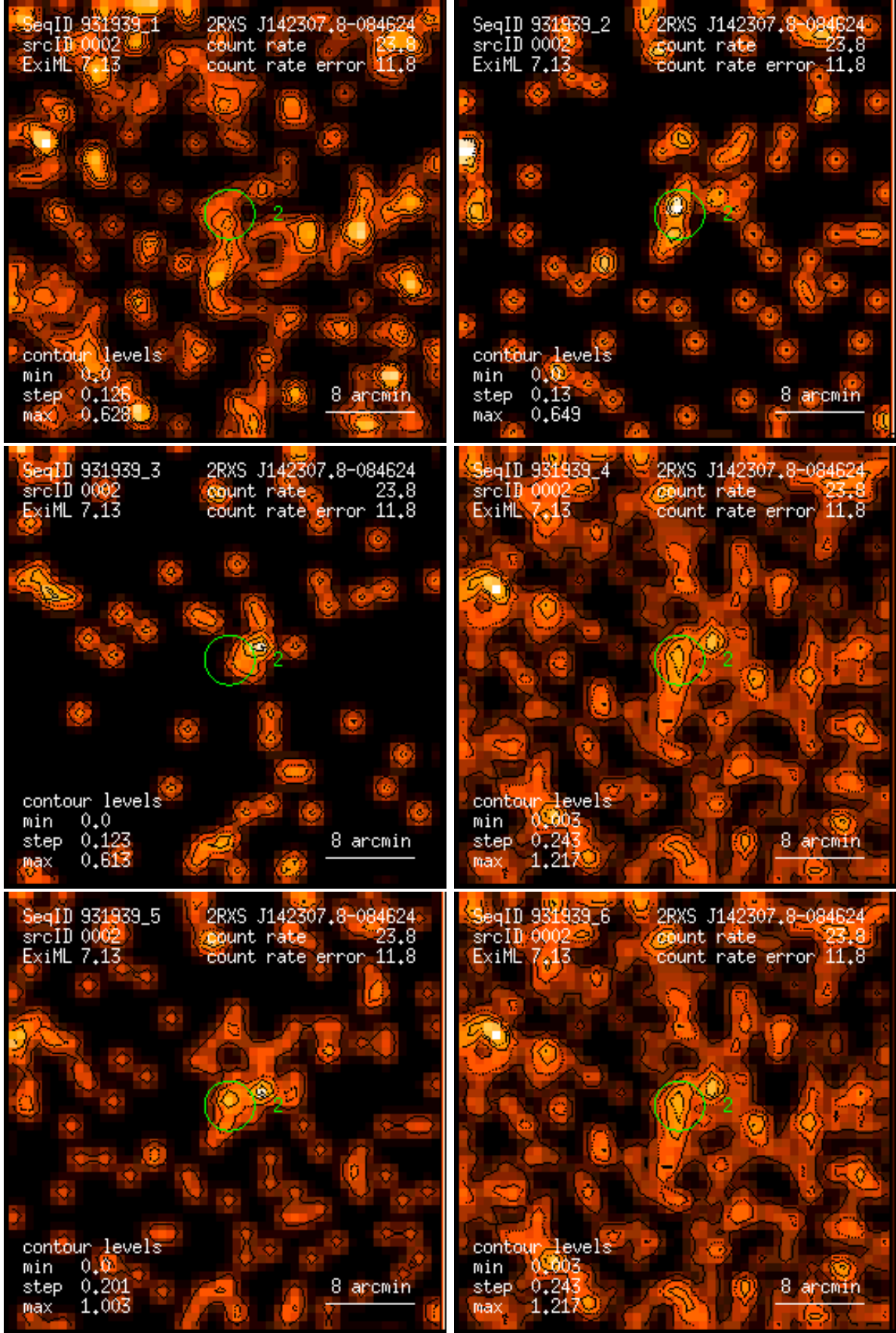
Figure 2: RASS 931939: detection 0002: band rate images, Gaussian filter: (1) PSPC channels 11 – 41, (2) 52 – 90, (3) 91 – 201, (4) 11 – 235, (5) 52 – 201, (6) 11 – 201. Broad band rates in counts/ks. Band rate contour levels in counts/ks/arcmin 2 .
