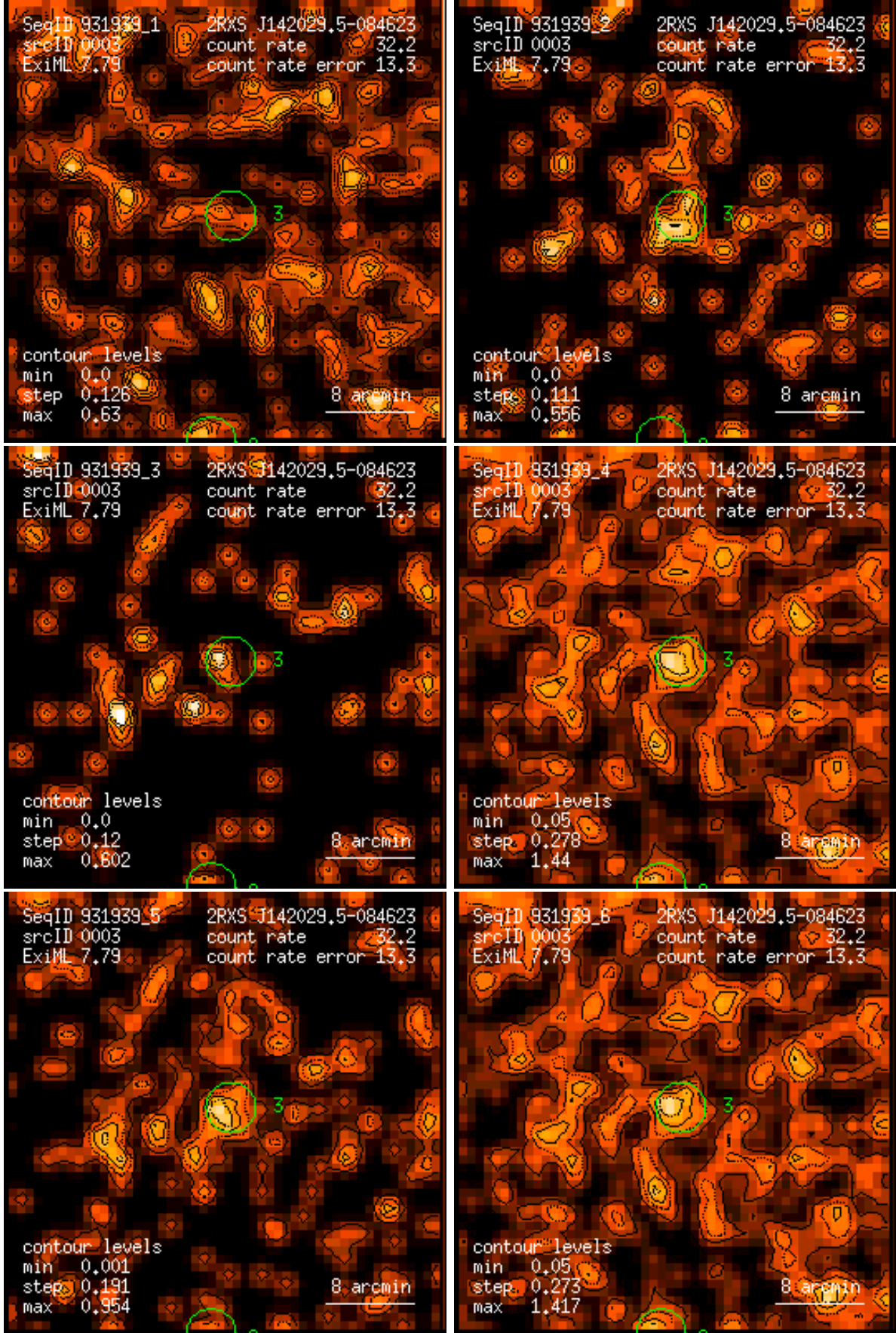
Figure 3: RASS 931939: detection 0003: band rate images, Gaussian filter: (1) PSPC channels 11 – 41, (2) 52 – 90, (3) 91 – 201, (4) 11 – 235, (5) 52 – 201, (6) 11 – 201. Broad band rates in counts/ks. Band rate contour levels in counts/ks/arcmin 2 .
