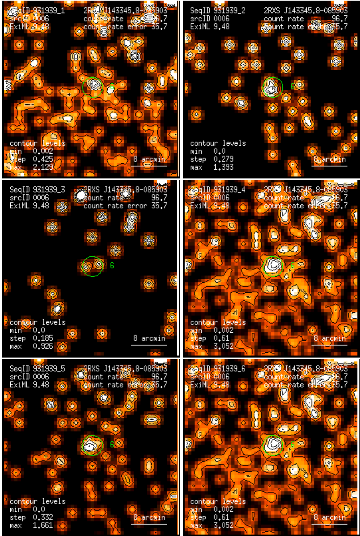
Figure 6: RASS 931939: detection 0006: band rate images, Gaussian filter: (1) PSPC channels 11 – 41, (2) 52 – 90, (3) 91 – 201, (4) 11 – 235, (5) 52 – 201, (6) 11 – 201. Broad band rates in counts/ks. Band rate contour levels in counts/ks/arcmin 2 .
