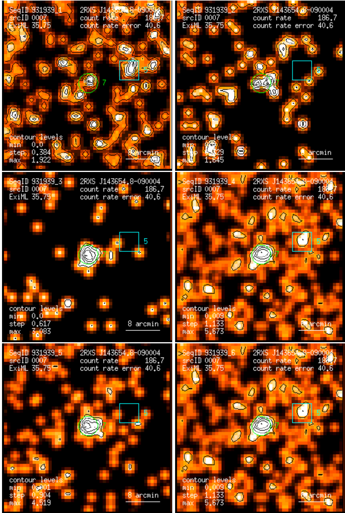
Figure 7: RASS 931939: detection 0007: band rate images, Gaussian filter: (1) PSPC channels 11 – 41, (2) 52 – 90, (3) 91 – 201, (4) 11 – 235, (5) 52 – 201, (6) 11 – 201. Broad band rates in counts/ks. Band rate contour levels in counts/ks/arcmin 2 .
