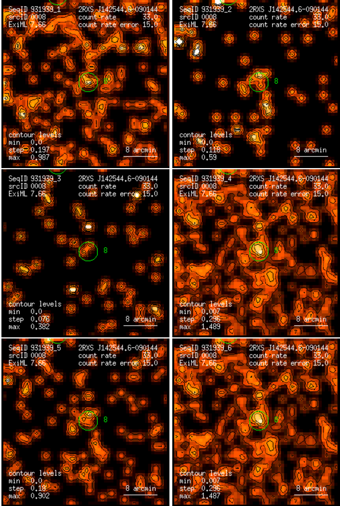
Figure 8: RASS 931939: detection 0008: band rate images, Gaussian filter: (1) PSPC channels 11 – 41, (2) 52 – 90, (3) 91 – 201, (4) 11 – 235, (5) 52 – 201, (6) 11 – 201. Broad band rates in counts/ks. Band rate contour levels in counts/ks/arcmin 2 .
