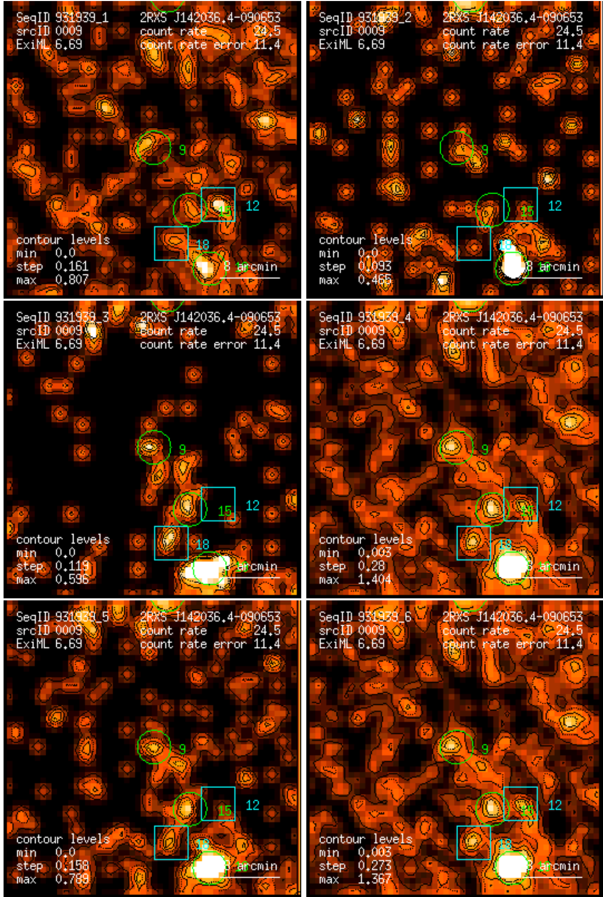
Figure 9: RASS 931939: detection 0009: band rate images, Gaussian filter: (1) PSPC channels 11 – 41, (2) 52 – 90, (3) 91 – 201, (4) 11 – 235, (5) 52 – 201, (6) 11 – 201. Broad band rates in counts/ks. Band rate contour levels in counts/ks/arcmin 2 .
