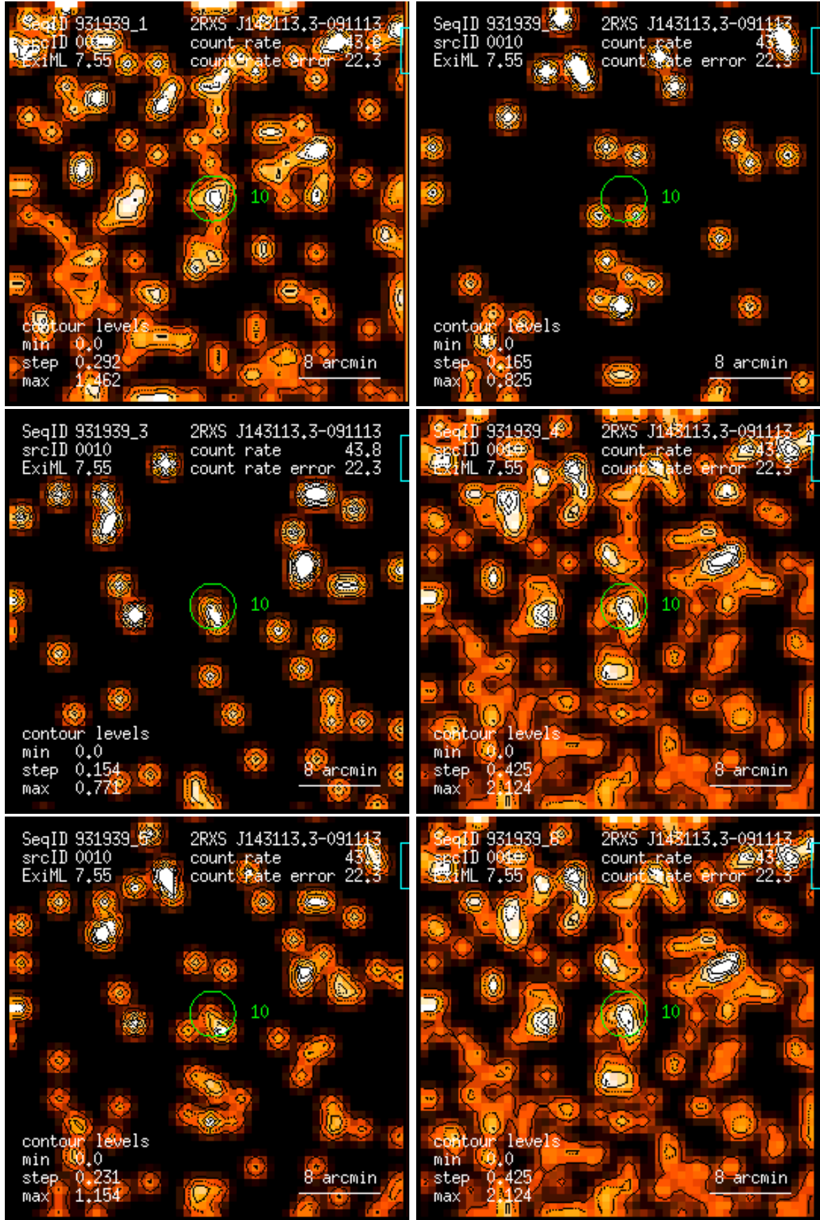
Figure 10: RASS 931939: detection 0010: band rate images, Gaussian filter: (1) PSPC channels 11 – 41, (2) 52 – 90, (3) 91 – 201, (4) 11 – 235, (5) 52 – 201, (6) 11 – 201. Broad band rates in counts/ks. Band rate contour levels in counts/ks/arcmin 2 .
