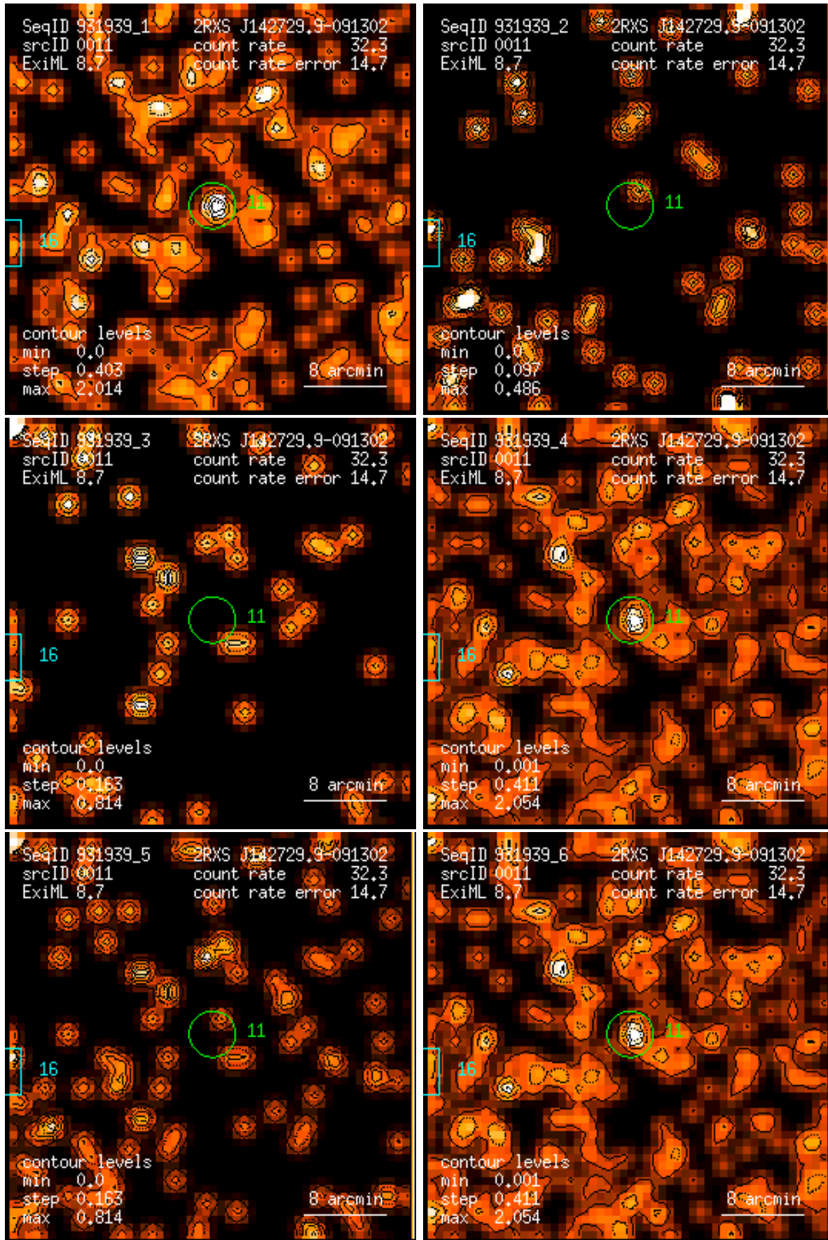
Figure 11: RASS 931939: detection 0011: band rate images, Gaussian filter: (1) PSPC channels 11 – 41, (2) 52 – 90, (3) 91 – 201, (4) 11 – 235, (5) 52 – 201, (6) 11 – 201. Broad band rates in counts/ks. Band rate contour levels in counts/ks/arcmin 2 .
