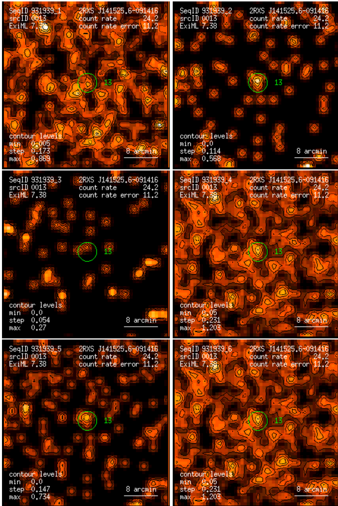
Figure 13: RASS 931939: detection 0013: band rate images, Gaussian filter: (1) PSPC channels 11 – 41, (2) 52 – 90, (3) 91 – 201, (4) 11 – 235, (5) 52 – 201, (6) 11 – 201. Broad band rates in counts/ks. Band rate contour levels in counts/ks/arcmin 2 .
