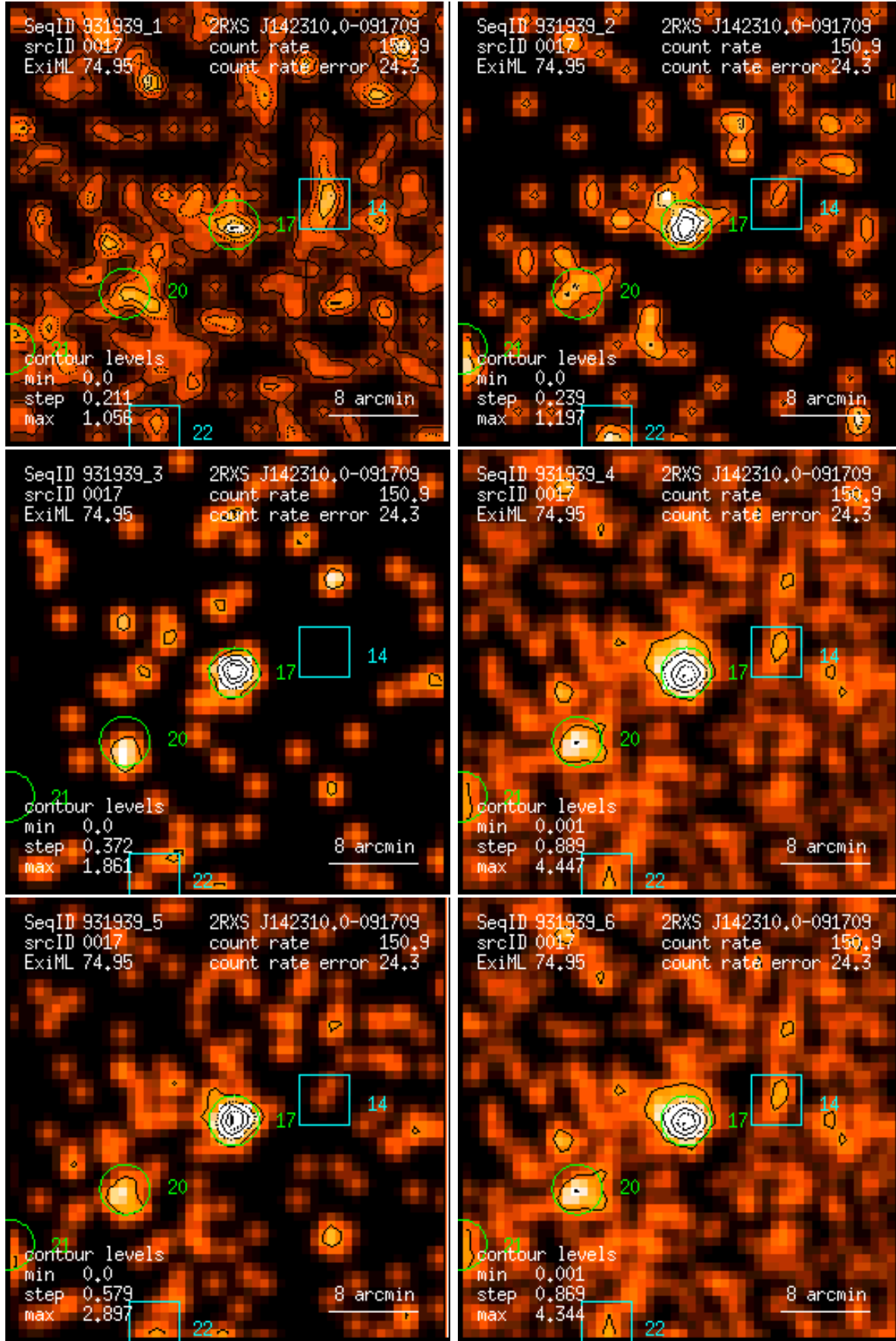
Figure 17: RASS 931939: detection 0017: band rate images, Gaussian filter: (1) PSPC channels 11 – 41, (2) 52 – 90, (3) 91 – 201, (4) 11 – 235, (5) 52 – 201, (6) 11 – 201. Broad band rates in counts/ks. Band rate contour levels in counts/ks/arcmin 2 .
