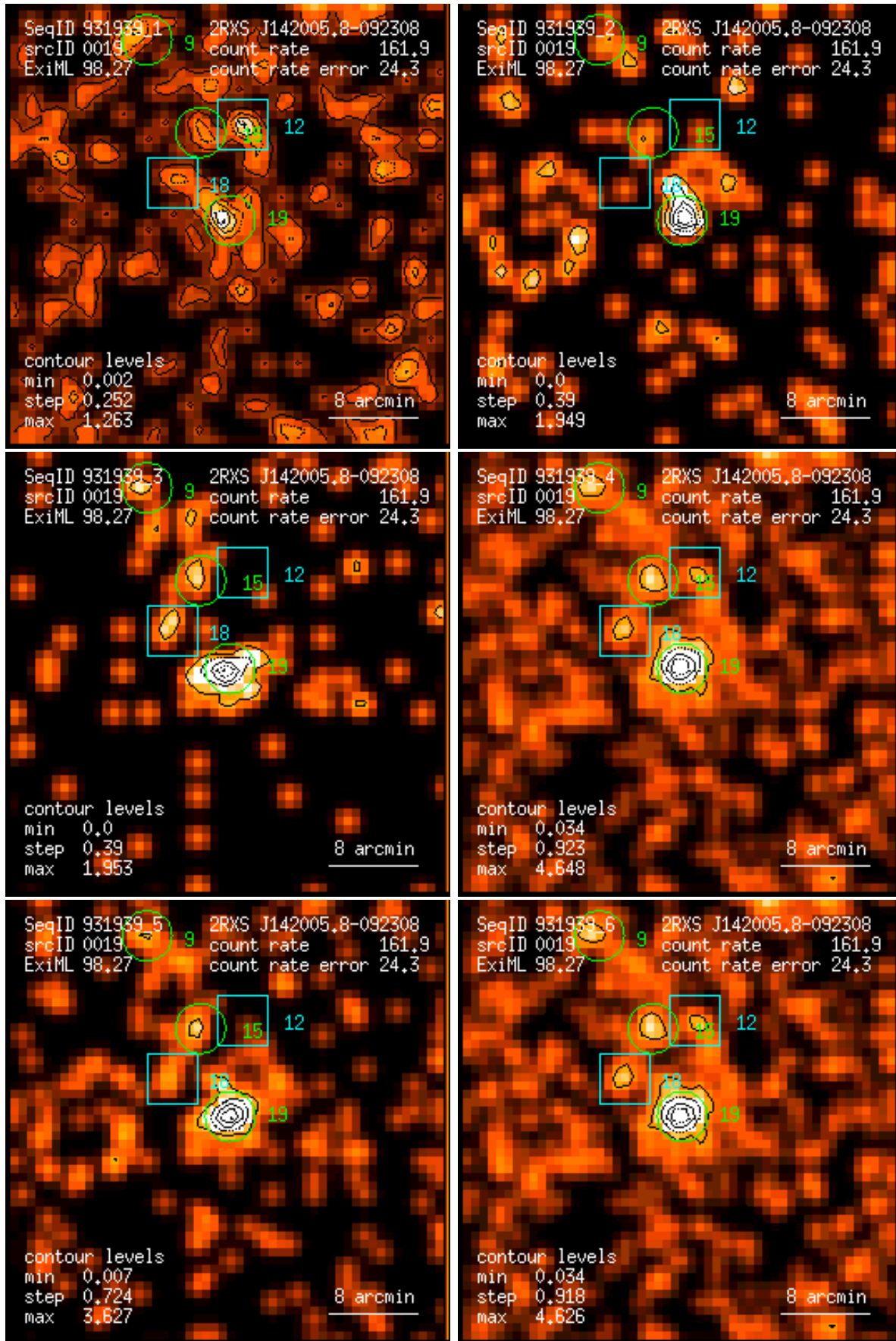
Figure 19: RASS 931939: detection 0019: band rate images, Gaussian filter: (1) PSPC channels 11 – 41, (2) 52 – 90, (3) 91 – 201, (4) 11 – 235, (5) 52 – 201, (6) 11 – 201. Broad band rates in counts/ks. Band rate contour levels in counts/ks/arcmin 2 .
