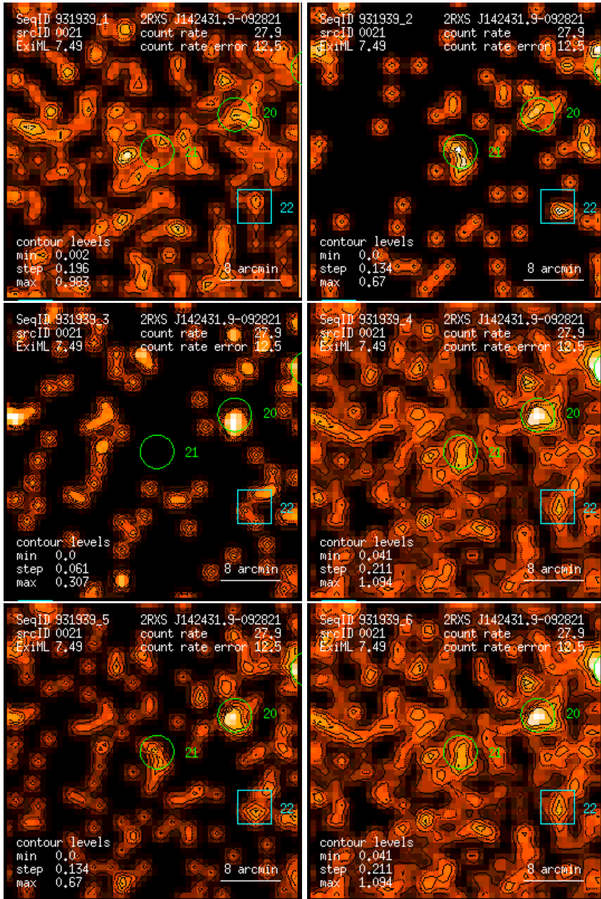
Figure 21: RASS 931939: detection 0021: band rate images, Gaussian filter: (1) PSPC channels 11 – 41, (2) 52 – 90, (3) 91 – 201, (4) 11 – 235, (5) 52 – 201, (6) 11 – 201. Broad band rates in counts/ks. Band rate contour levels in counts/ks/arcmin 2 .
