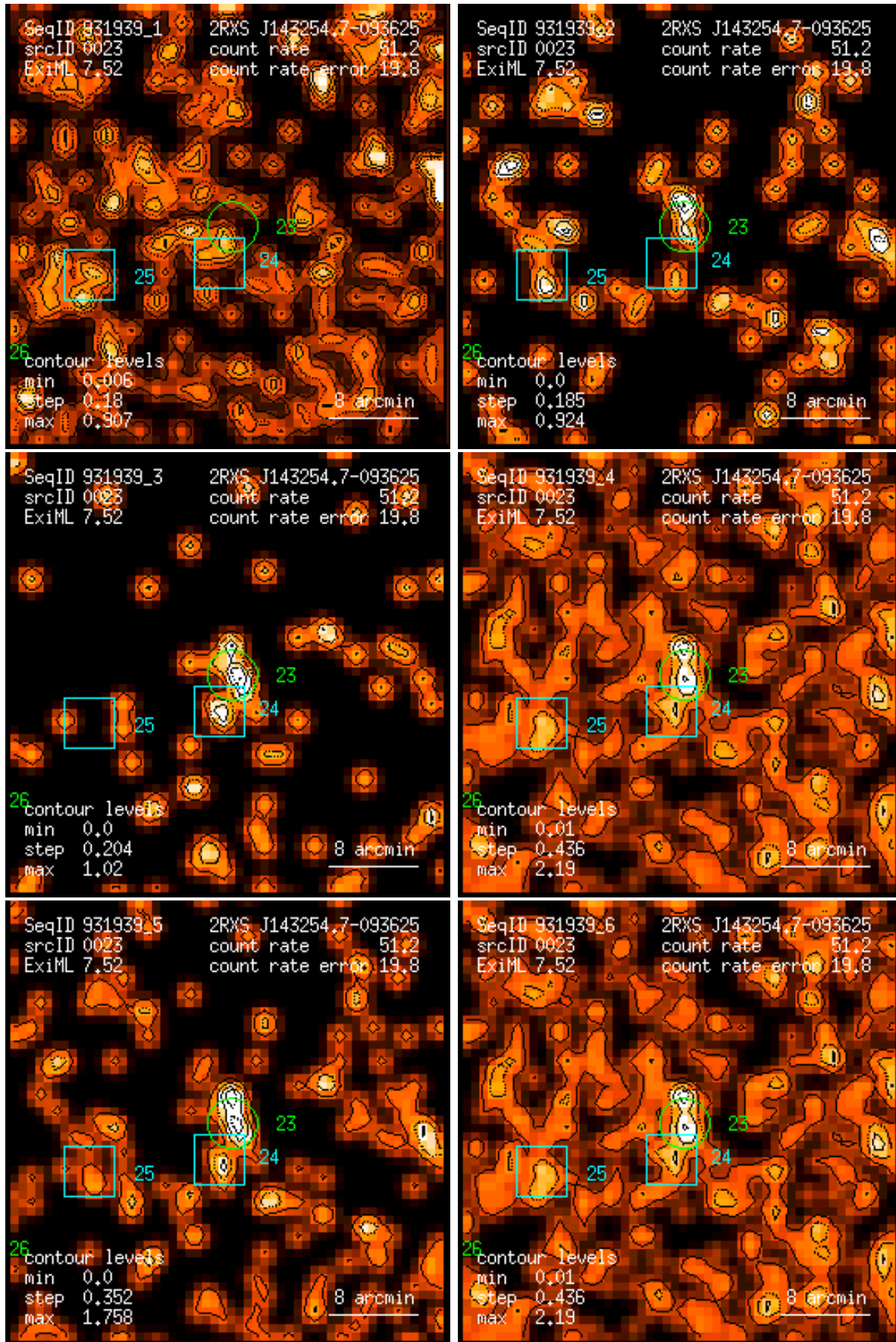
Figure 23: RASS 931939: detection 0023: band rate images, Gaussian filter: (1) PSPC channels 11 – 41, (2) 52 – 90, (3) 91 – 201, (4) 11 – 235, (5) 52 – 201, (6) 11 – 201. Broad band rates in counts/ks. Band rate contour levels in counts/ks/arcmin 2 .
