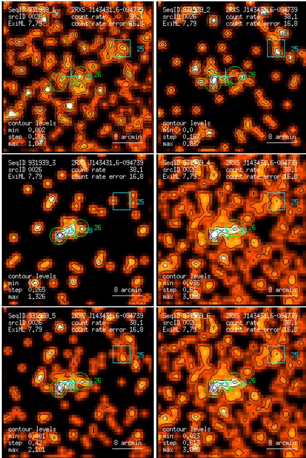
Figure 26: RASS 931939: detection 0026: band rate images, Gaussian filter: (1) PSPC channels 11 – 41, (2) 52 – 90, (3) 91 – 201, (4) 11 – 235, (5) 52 – 201, (6) 11 – 201. Broad band rates in counts/ks. Band rate contour levels in counts/ks/arcmin 2 .
