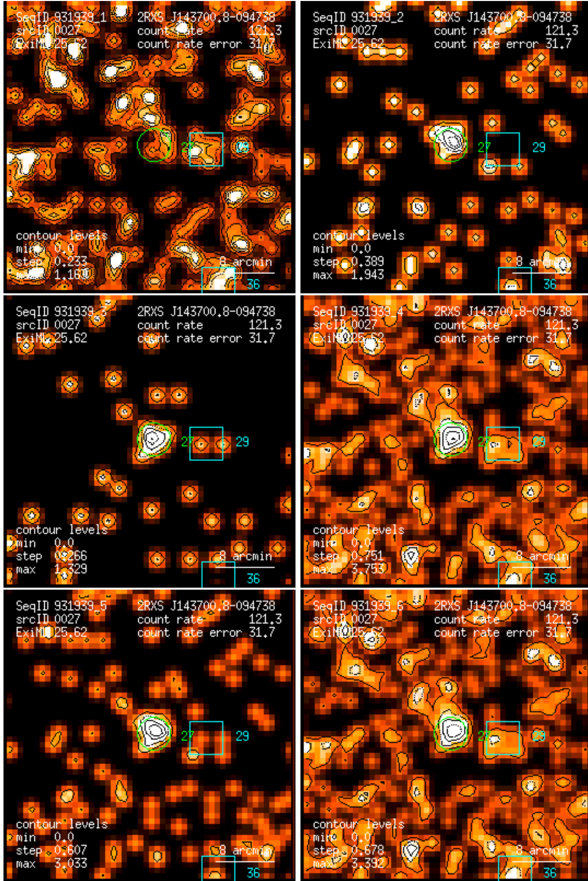
Figure 27: RASS 931939: detection 0027: band rate images, Gaussian filter: (1) PSPC channels 11 – 41, (2) 52 – 90, (3) 91 – 201, (4) 11 – 235, (5) 52 – 201, (6) 11 – 201. Broad band rates in counts/ks. Band rate contour levels in counts/ks/arcmin 2 .
