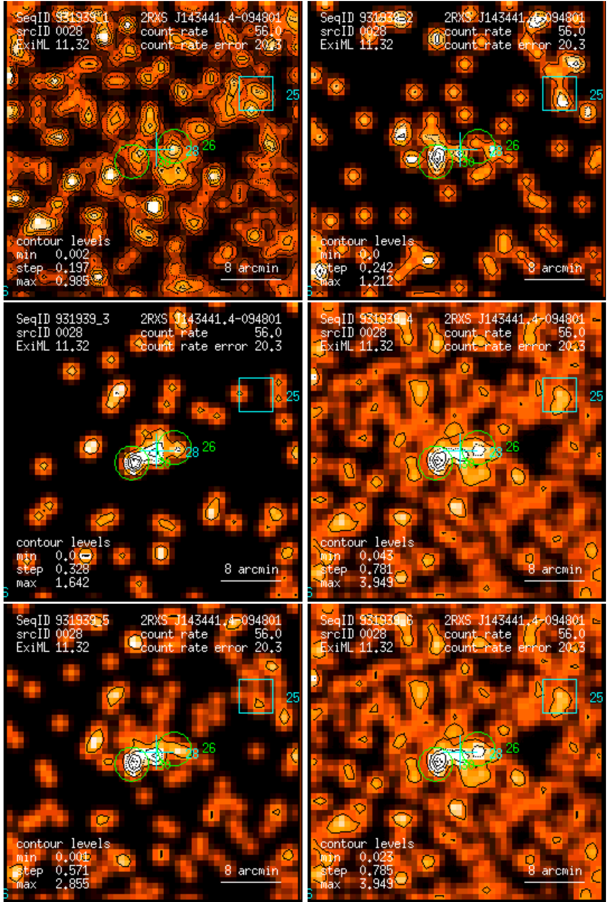
Figure 28: RASS 931939: detection 0028: band rate images, Gaussian filter: (1) PSPC channels 11 – 41, (2) 52 – 90, (3) 91 – 201, (4) 11 – 235, (5) 52 – 201, (6) 11 – 201. Broad band rates in counts/ks. Band rate contour levels in counts/ks/arcmin 2 .
