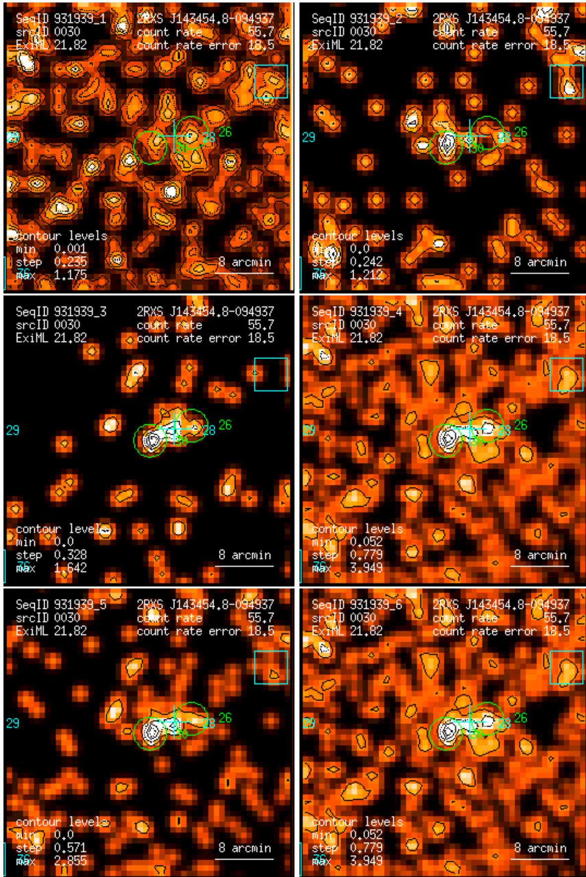
Figure 30: RASS 931939: detection 0030: band rate images, Gaussian filter: (1) PSPC channels 11 – 41, (2) 52 – 90, (3) 91 – 201, (4) 11 – 235, (5) 52 – 201, (6) 11 – 201. Broad band rates in counts/ks. Band rate contour levels in counts/ks/arcmin 2 .
