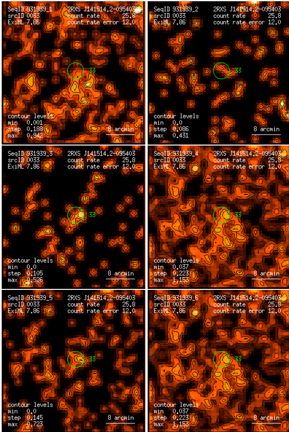
Figure 33: RASS 931939: detection 0033: band rate images, Gaussian filter: (1) PSPC channels 11 – 41, (2) 52 – 90, (3) 91 – 201, (4) 11 – 235, (5) 52 – 201, (6) 11 – 201. Broad band rates in counts/ks. Band rate contour levels in counts/ks/arcmin 2 .
