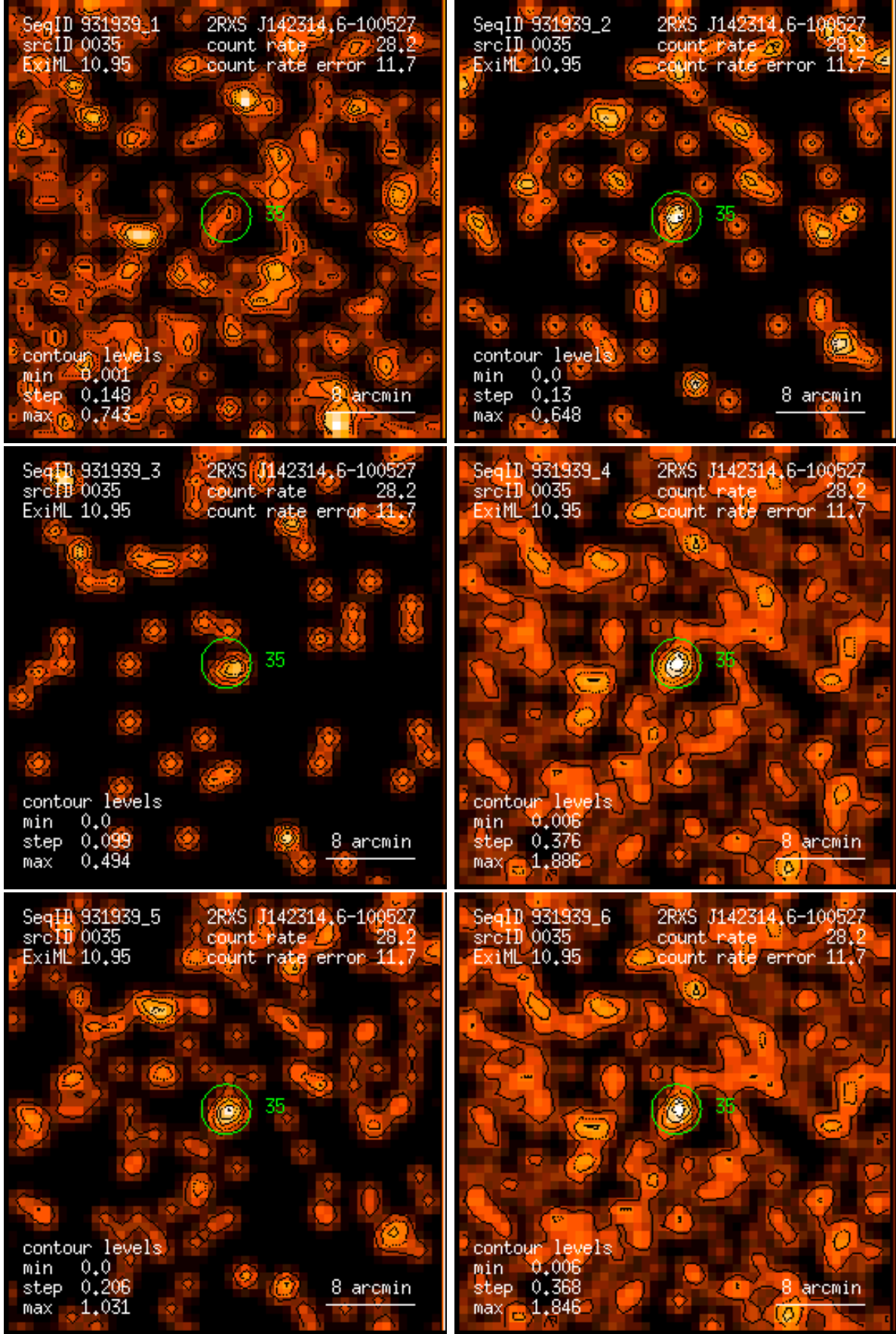
Figure 35: RASS 931939: detection 0035: band rate images, Gaussian filter: (1) PSPC channels 11 – 41, (2) 52 – 90, (3) 91 – 201, (4) 11 – 235, (5) 52 – 201, (6) 11 – 201. Broad band rates in counts/ks. Band rate contour levels in counts/ks/arcmin 2 .
