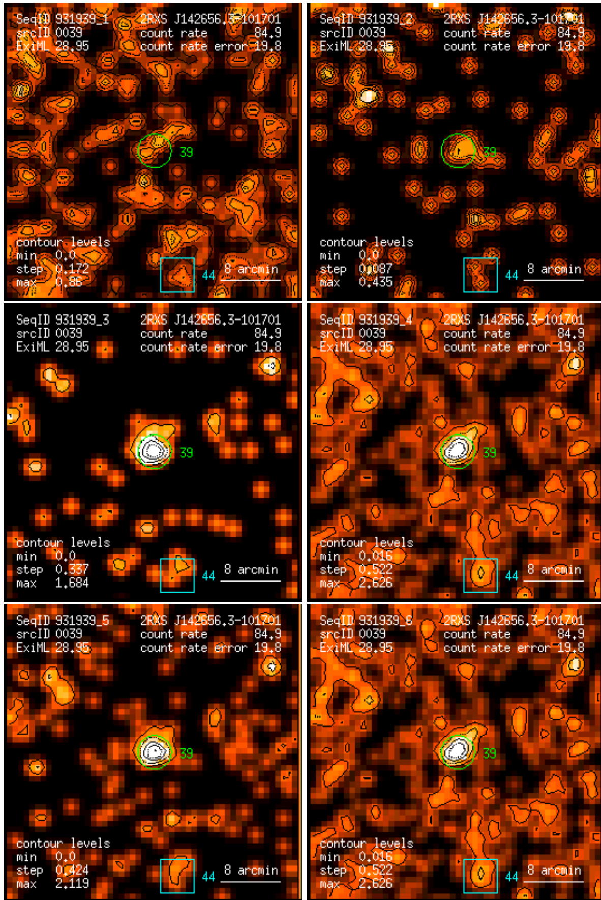
Figure 39: RASS 931939: detection 0039: band rate images, Gaussian filter: (1) PSPC channels 11 – 41, (2) 52 – 90, (3) 91 – 201, (4) 11 – 235, (5) 52 – 201, (6) 11 – 201. Broad band rates in counts/ks. Band rate contour levels in counts/ks/arcmin 2 .
