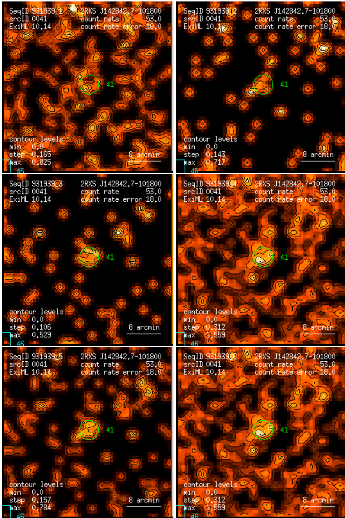
Figure 41: RASS 931939: detection 0041: band rate images, Gaussian filter: (1) PSPC channels 11 – 41, (2) 52 – 90, (3) 91 – 201, (4) 11 – 235, (5) 52 – 201, (6) 11 – 201. Broad band rates in counts/ks. Band rate contour levels in counts/ks/arcmin 2 .
