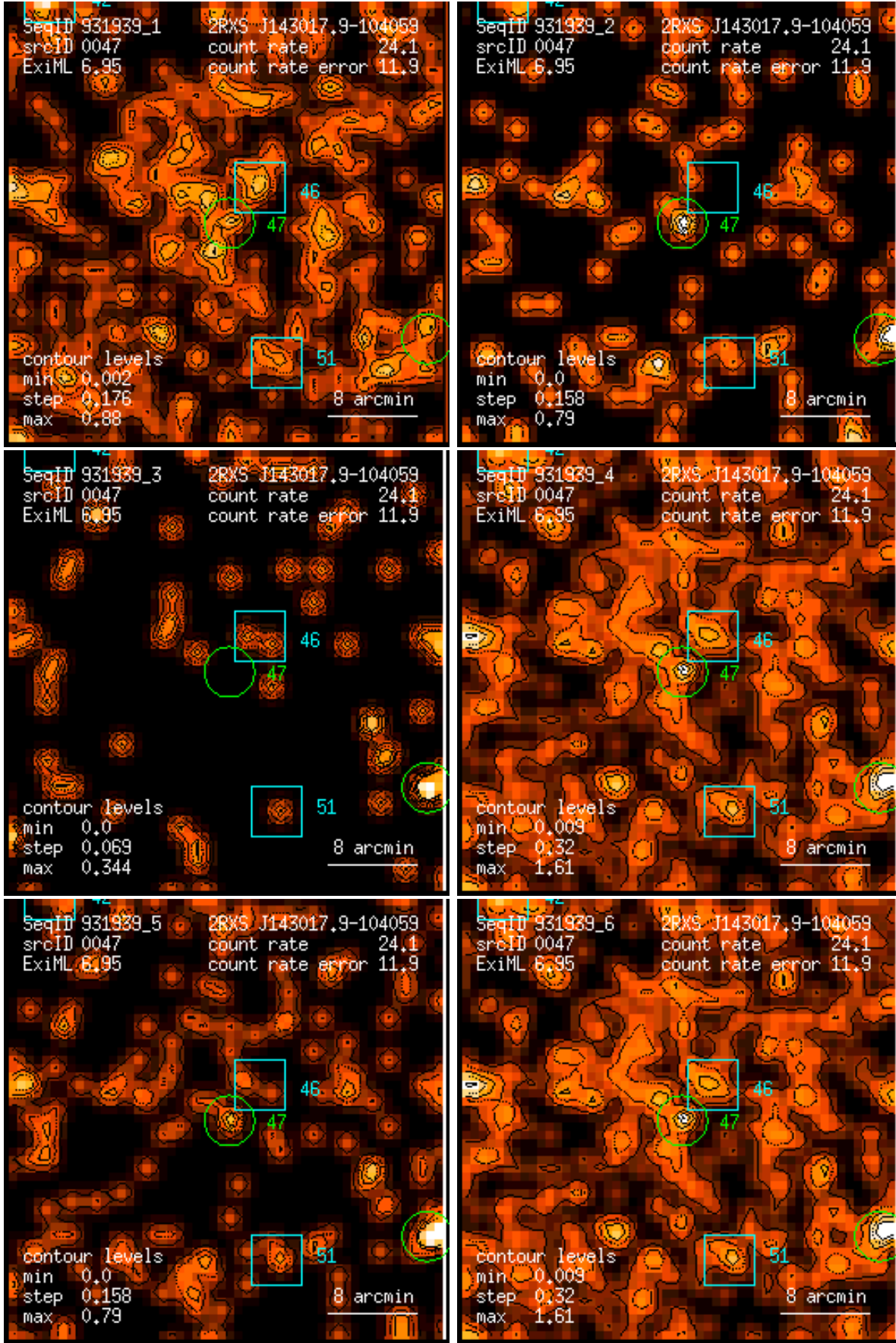
Figure 47: RASS 931939: detection 0047: band rate images, Gaussian filter: (1) PSPC channels 11 – 41, (2) 52 – 90, (3) 91 – 201, (4) 11 – 235, (5) 52 – 201, (6) 11 – 201. Broad band rates in counts/ks. Band rate contour levels in counts/ks/arcmin 2 .
