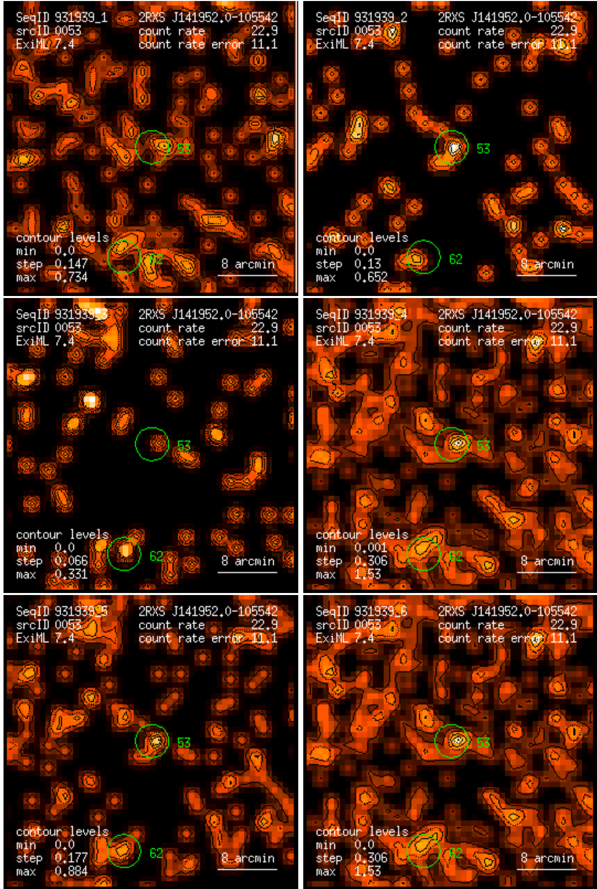
Figure 53: RASS 931939: detection 0053: band rate images, Gaussian filter: (1) PSPC channels 11 – 41, (2) 52 – 90, (3) 91 – 201, (4) 11 – 235, (5) 52 – 201, (6) 11 – 201. Broad band rates in counts/ks. Band rate contour levels in counts/ks/arcmin 2 .
