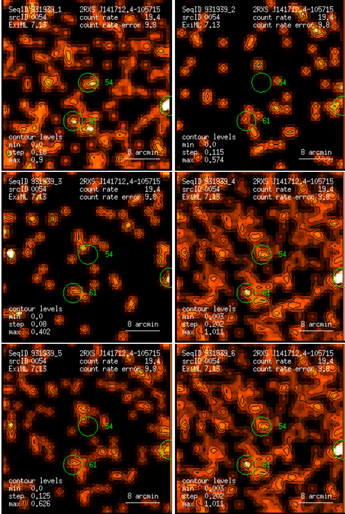
Figure 54: RASS 931939: detection 0054: band rate images, Gaussian filter: (1) PSPC channels 11 – 41, (2) 52 – 90, (3) 91 – 201, (4) 11 – 235, (5) 52 – 201, (6) 11 – 201. Broad band rates in counts/ks. Band rate contour levels in counts/ks/arcmin 2 .
