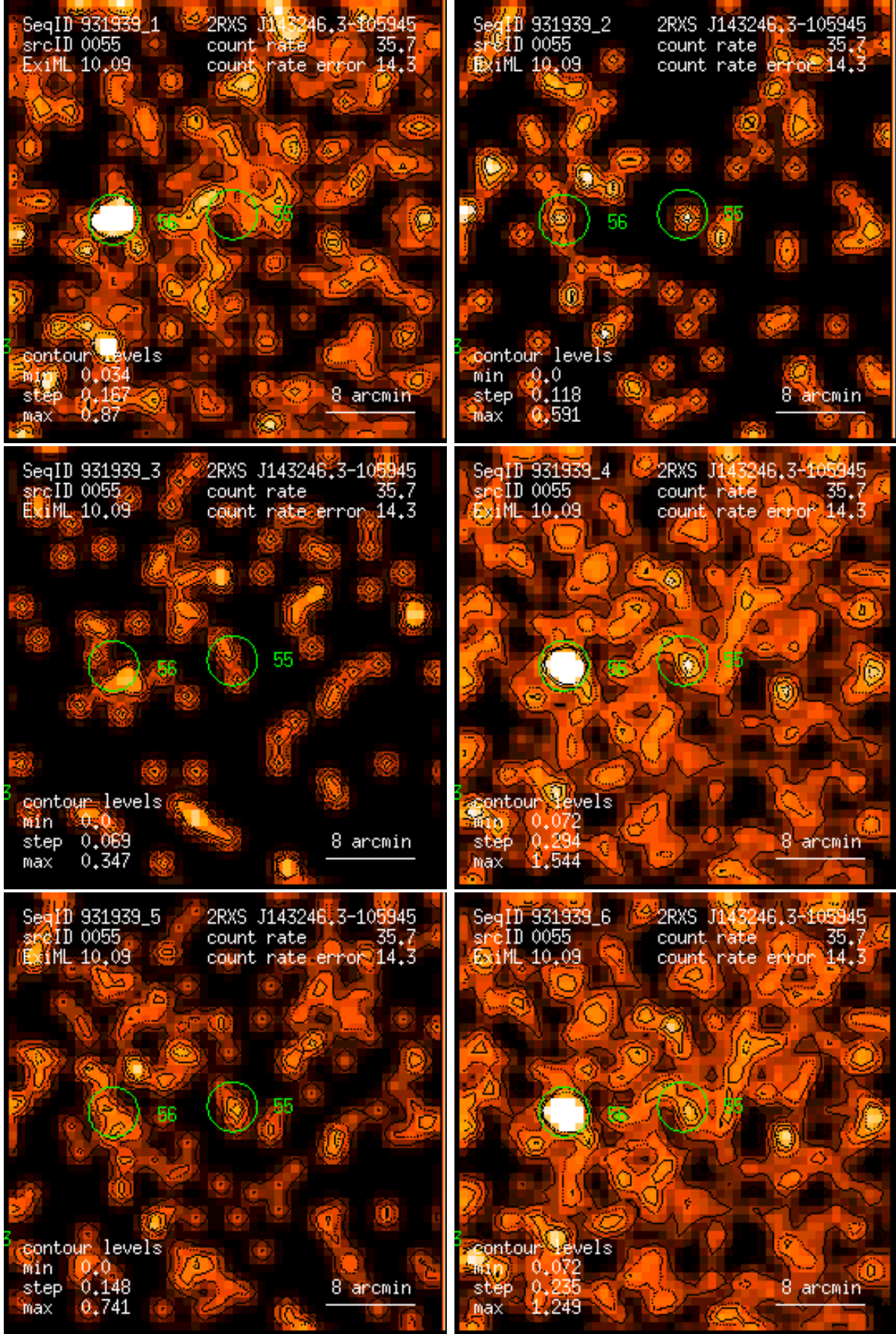
Figure 55: RASS 931939: detection 0055: band rate images, Gaussian filter: (1) PSPC channels 11 – 41, (2) 52 – 90, (3) 91 – 201, (4) 11 – 235, (5) 52 – 201, (6) 11 – 201. Broad band rates in counts/ks. Band rate contour levels in counts/ks/arcmin 2 .
