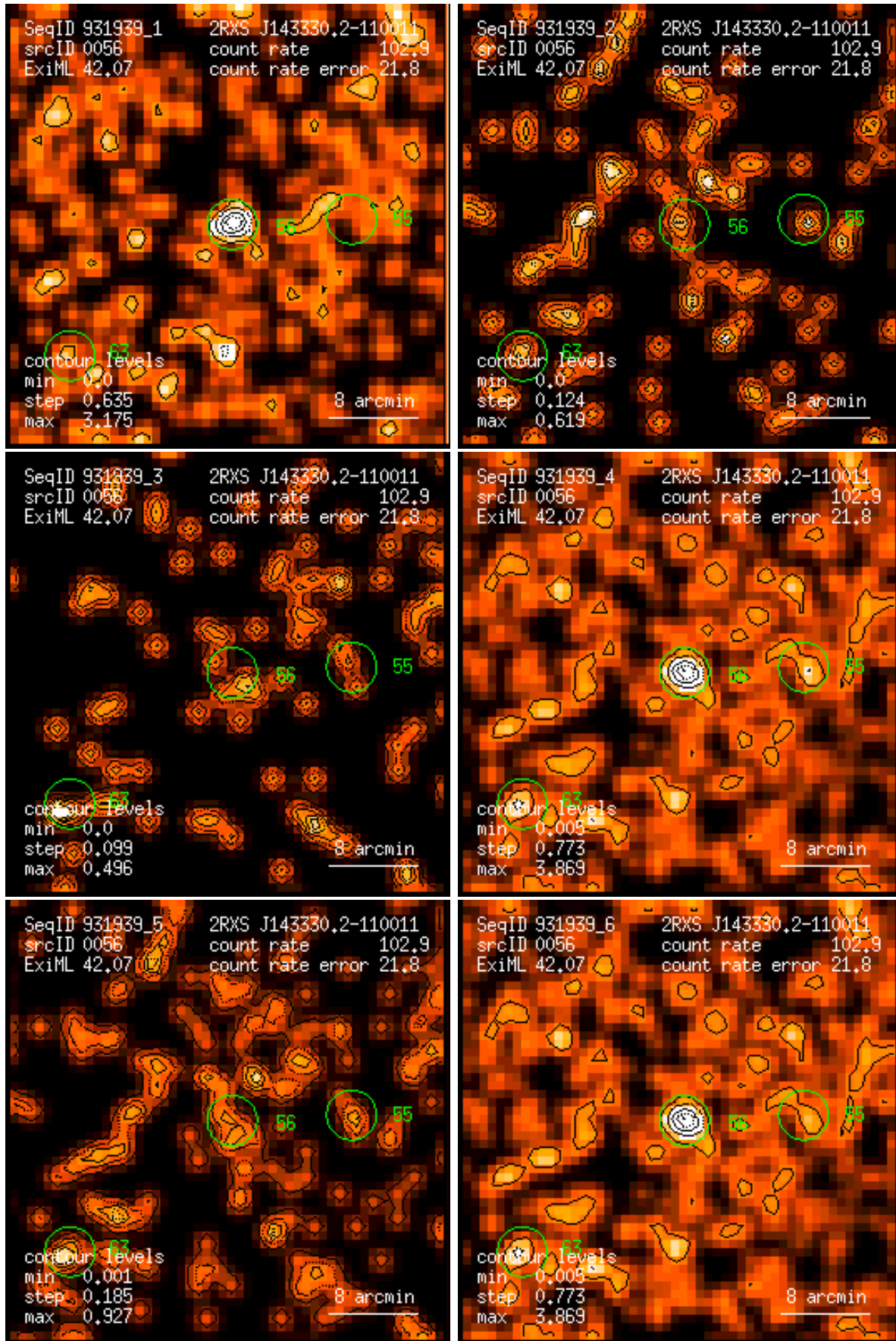
Figure 56: RASS 931939: detection 0056: band rate images, Gaussian filter: (1) PSPC channels 11 – 41, (2) 52 – 90, (3) 91 – 201, (4) 11 – 235, (5) 52 – 201, (6) 11 – 201. Broad band rates in counts/ks. Band rate contour levels in counts/ks/arcmin 2 .
