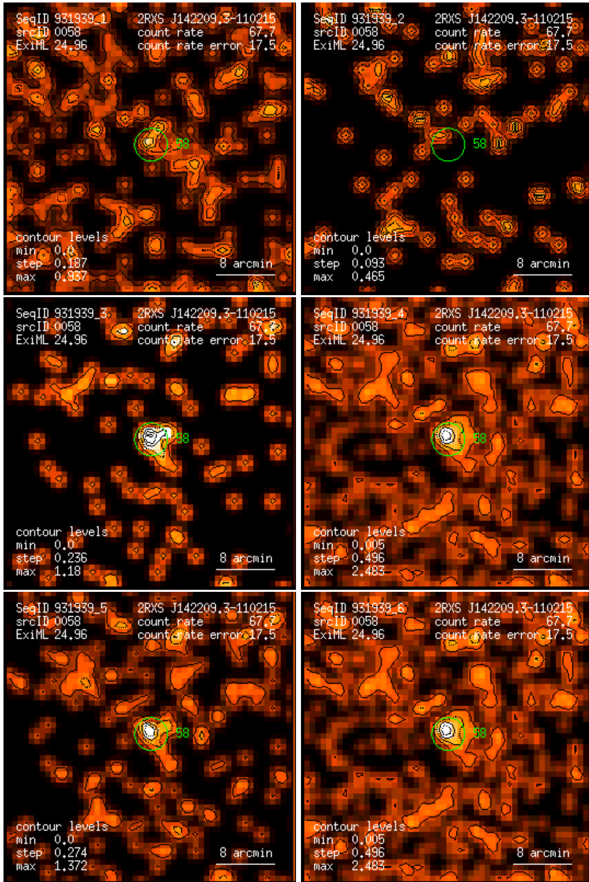
Figure 58: RASS 931939: detection 0058: band rate images, Gaussian filter: (1) PSPC channels 11 – 41, (2) 52 – 90, (3) 91 – 201, (4) 11 – 235, (5) 52 – 201, (6) 11 – 201. Broad band rates in counts/ks. Band rate contour levels in counts/ks/arcmin 2 .
