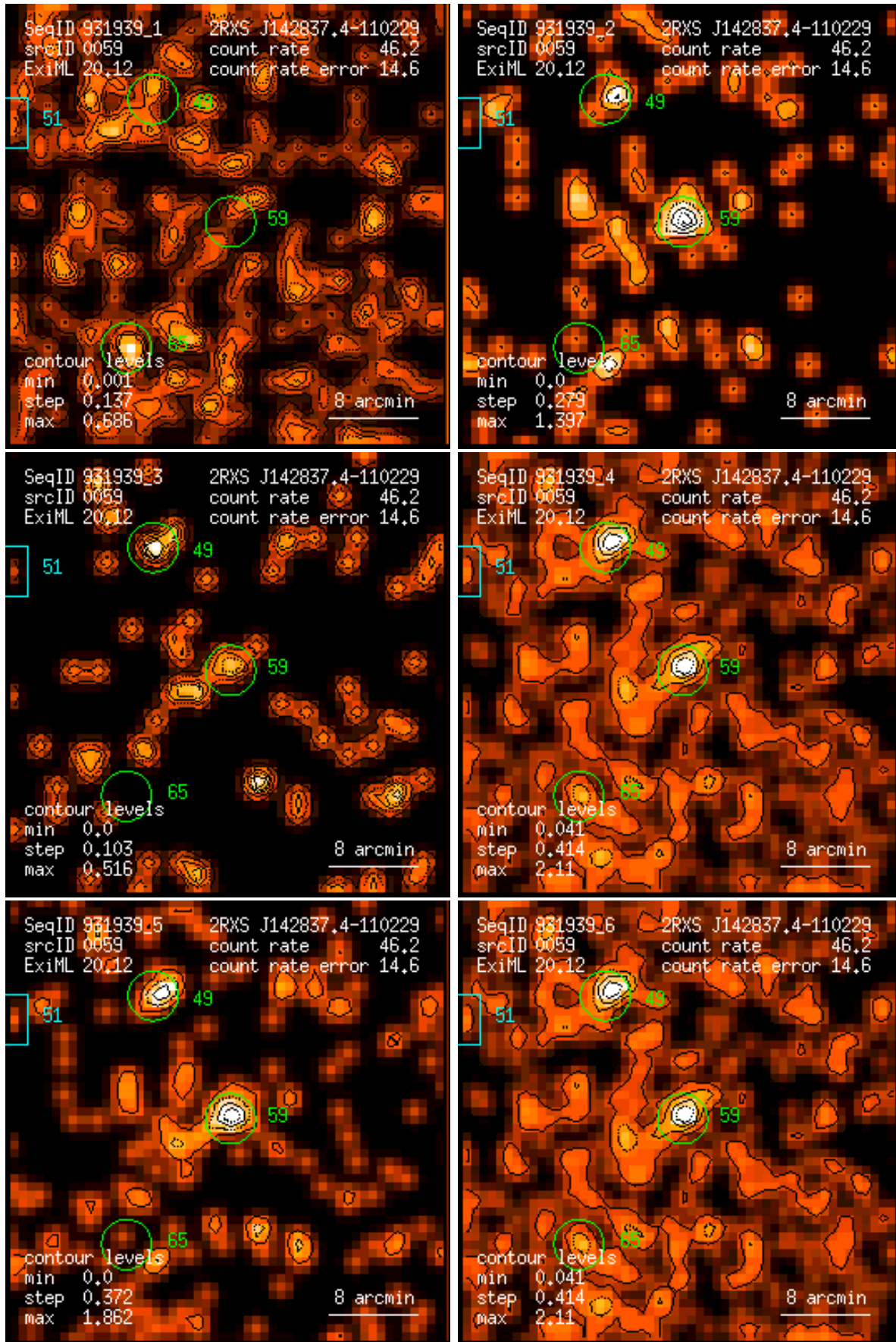
Figure 59: RASS 931939: detection 0059: band rate images, Gaussian filter: (1) PSPC channels 11 – 41, (2) 52 – 90, (3) 91 – 201, (4) 11 – 235, (5) 52 – 201, (6) 11 – 201. Broad band rates in counts/ks. Band rate contour levels in counts/ks/arcmin 2 .
