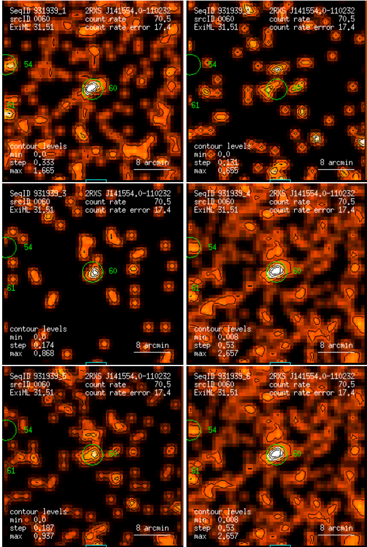
Figure 60: RASS 931939: detection 0060: band rate images, Gaussian filter: (1) PSPC channels 11 – 41, (2) 52 – 90, (3) 91 – 201, (4) 11 – 235, (5) 52 – 201, (6) 11 – 201. Broad band rates in counts/ks. Band rate contour levels in counts/ks/arcmin 2 .
