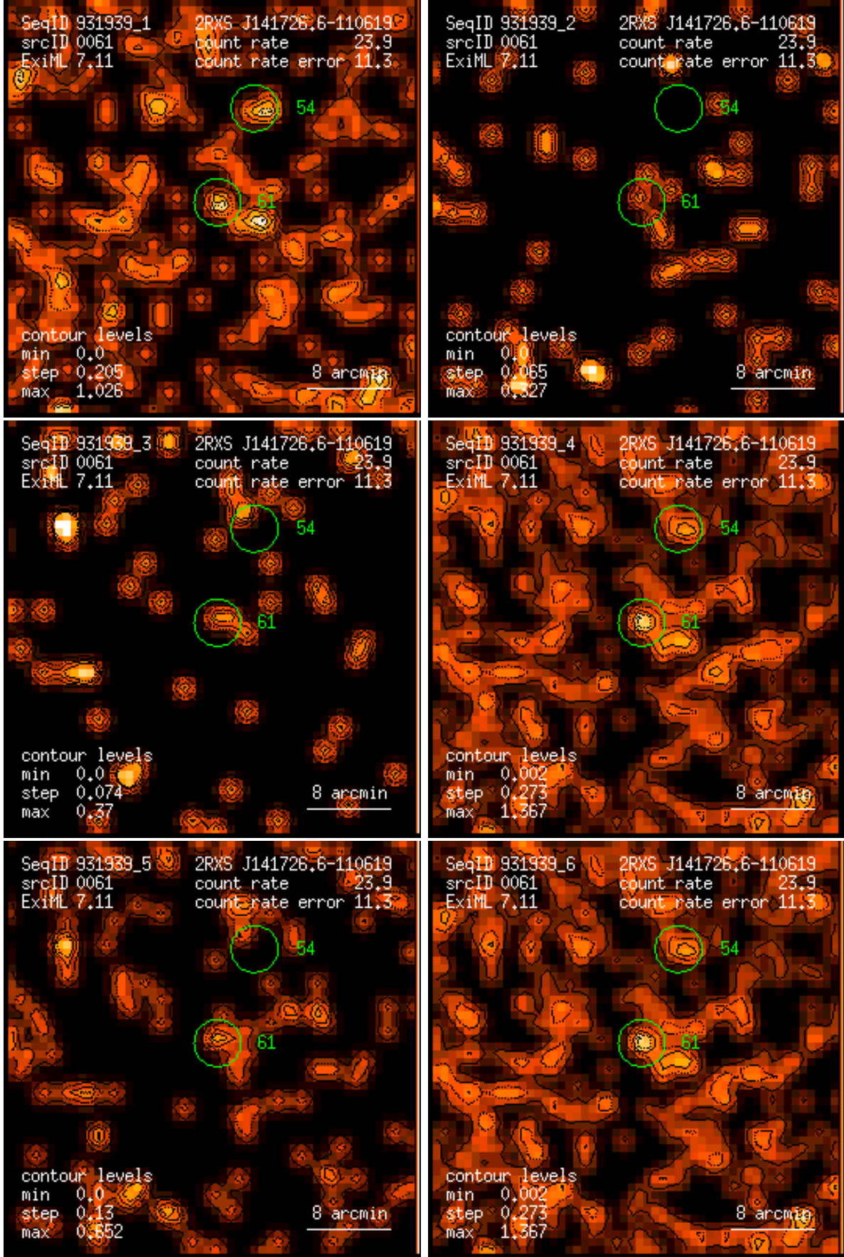
Figure 61: RASS 931939: detection 0061: band rate images, Gaussian filter: (1) PSPC channels 11 – 41, (2) 52 – 90, (3) 91 – 201, (4) 11 – 235, (5) 52 – 201, (6) 11 – 201. Broad band rates in counts/ks. Band rate contour levels in counts/ks/arcmin 2 .
