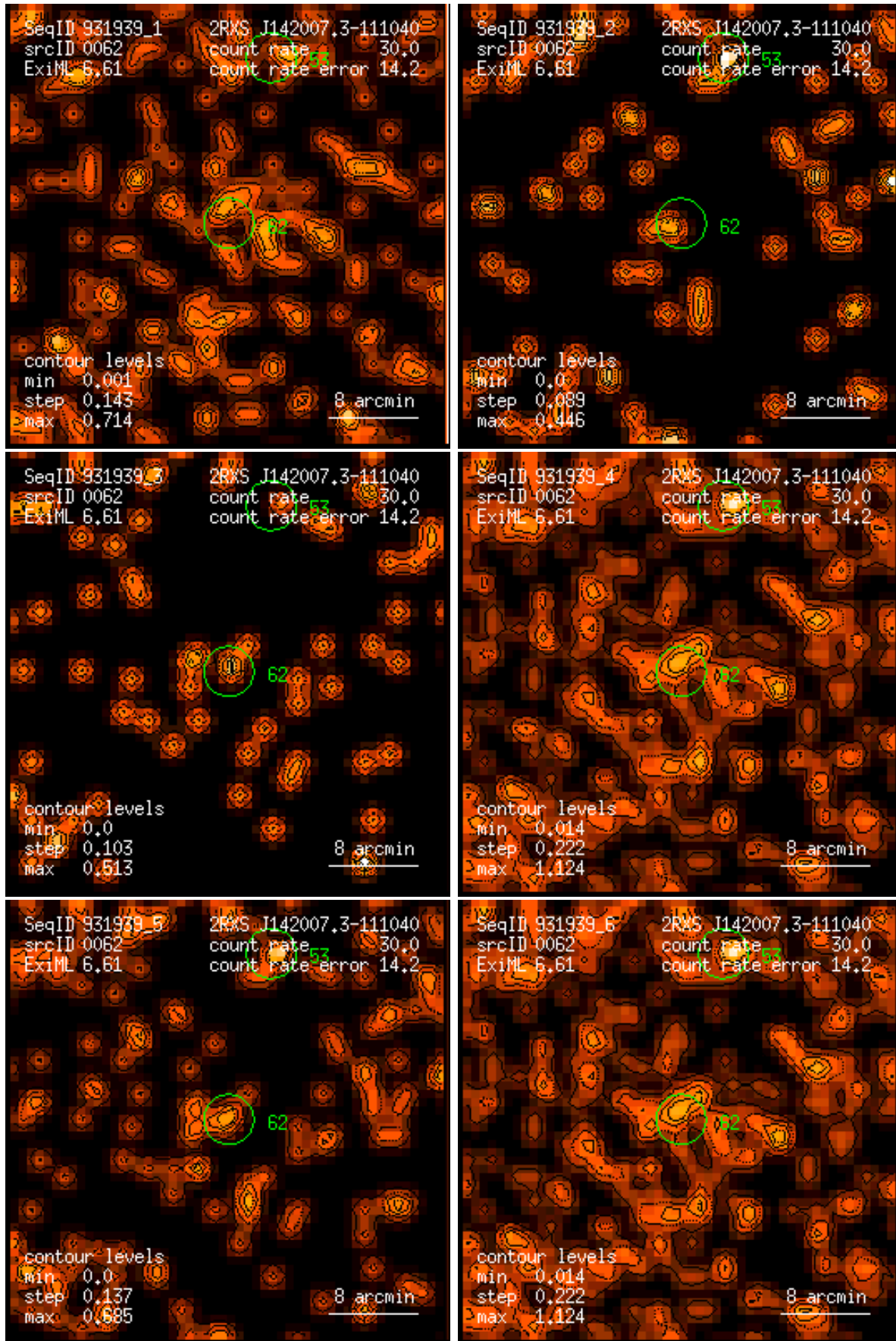
Figure 62: RASS 931939: detection 0062: band rate images, Gaussian filter: (1) PSPC channels 11 – 41, (2) 52 – 90, (3) 91 – 201, (4) 11 – 235, (5) 52 – 201, (6) 11 – 201. Broad band rates in counts/ks. Band rate contour levels in counts/ks/arcmin 2 .
