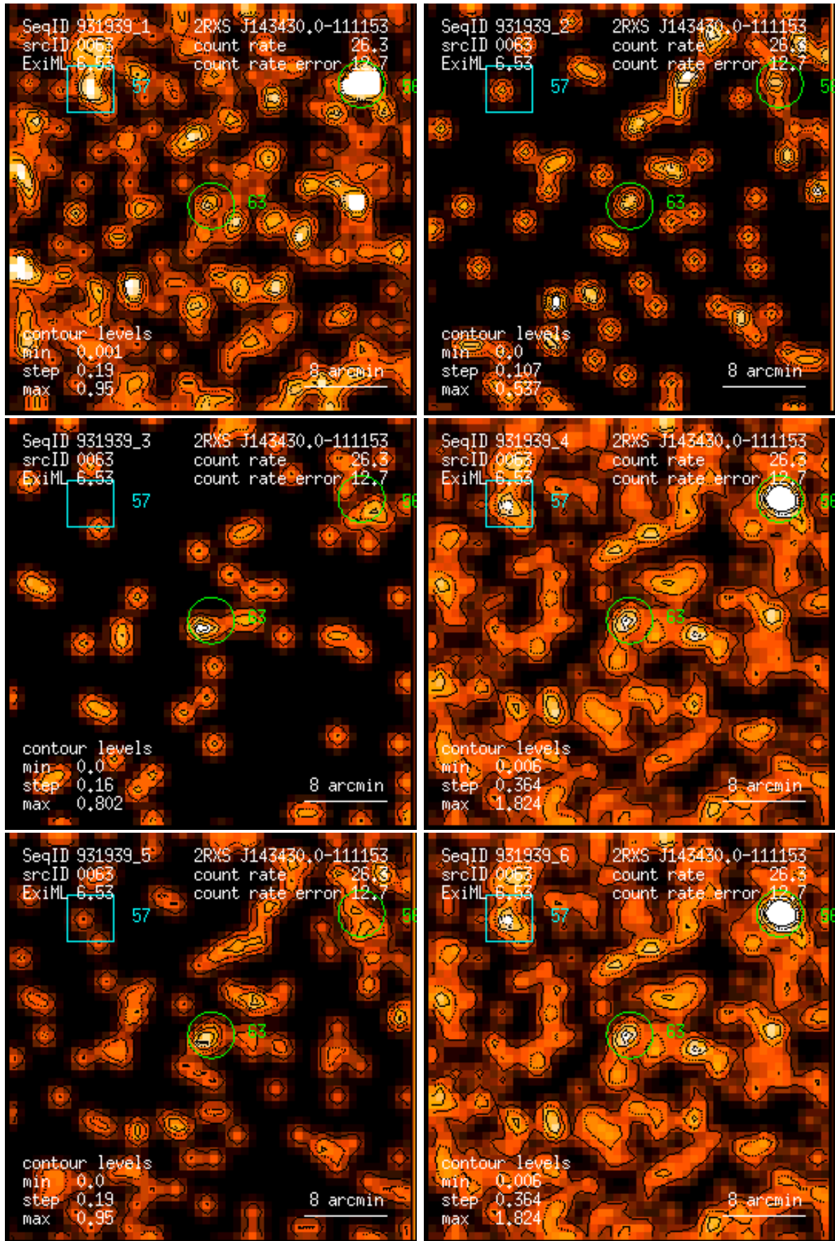
Figure 63: RASS 931939: detection 0063: band rate images, Gaussian filter: (1) PSPC channels 11 – 41, (2) 52 – 90, (3) 91 – 201, (4) 11 – 235, (5) 52 – 201, (6) 11 – 201. Broad band rates in counts/ks. Band rate contour levels in counts/ks/arcmin 2 .
