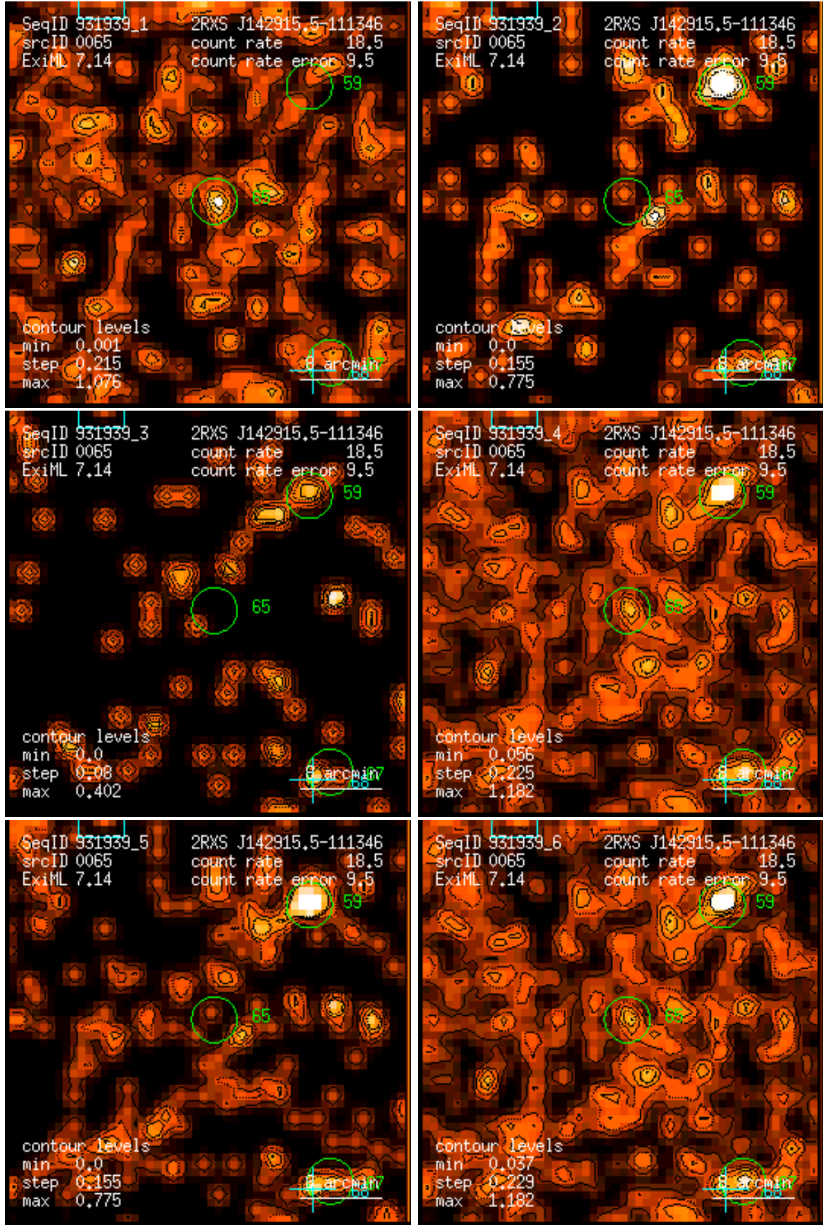
Figure 65: RASS 931939: detection 0065: band rate images, Gaussian filter: (1) PSPC channels 11 – 41, (2) 52 – 90, (3) 91 – 201, (4) 11 – 235, (5) 52 – 201, (6) 11 – 201. Broad band rates in counts/ks. Band rate contour levels in counts/ks/arcmin 2 .
