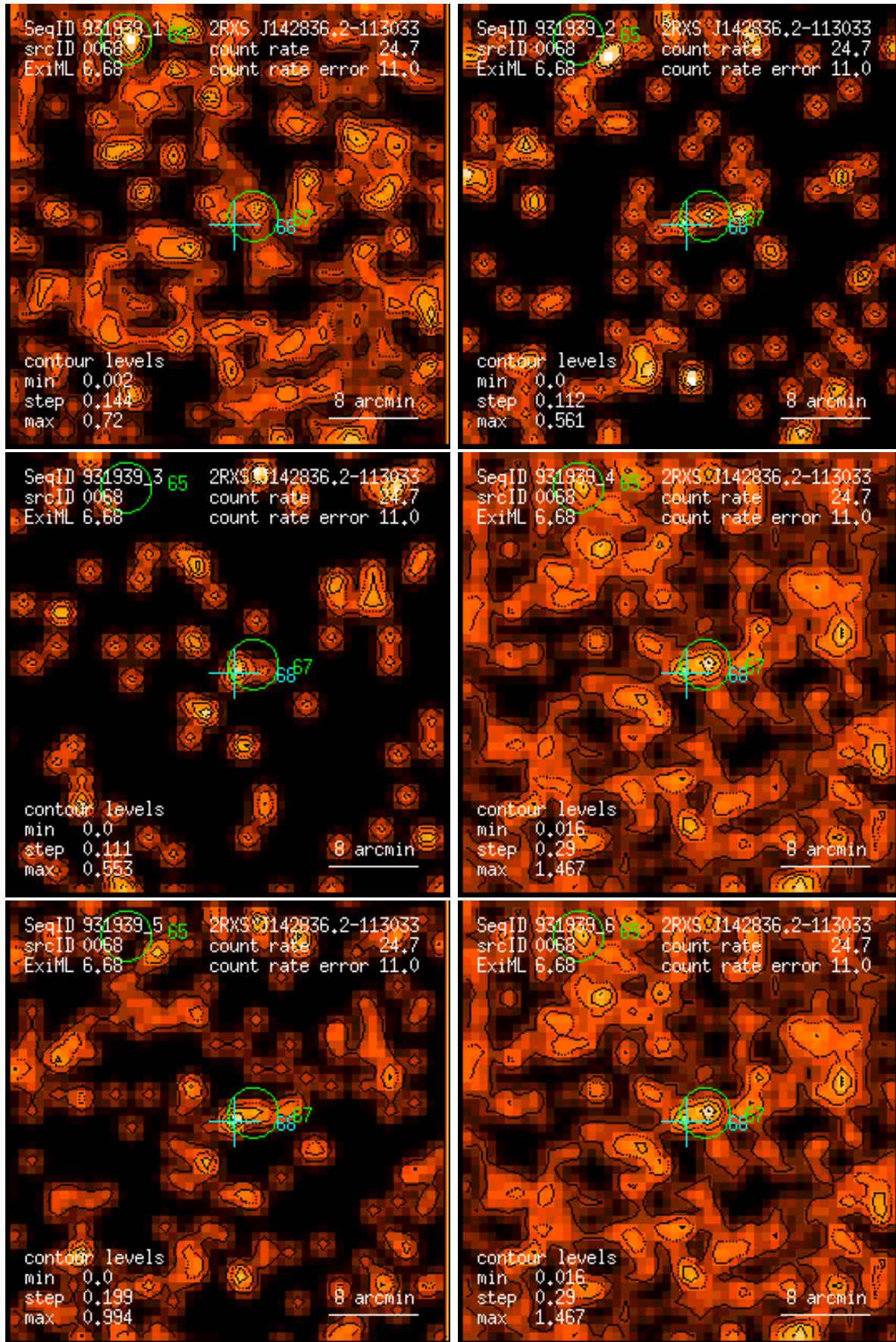
Figure 68: RASS 931939: detection 0068: band rate images, Gaussian filter: (1) PSPC channels 11 – 41, (2) 52 – 90, (3) 91 – 201, (4) 11 – 235, (5) 52 – 201, (6) 11 – 201. Broad band rates in counts/ks. Band rate contour levels in counts/ks/arcmin 2 .
