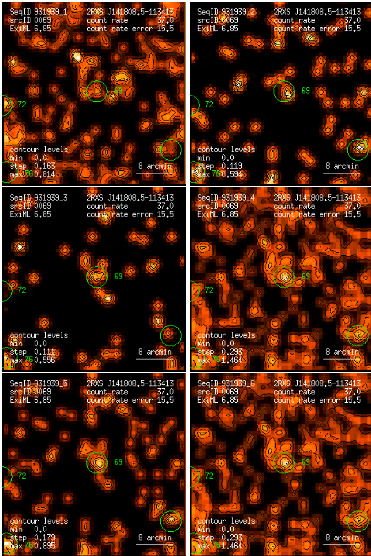
Figure 69: RASS 931939: detection 0069: band rate images, Gaussian filter: (1) PSPC channels 11 – 41, (2) 52 – 90, (3) 91 – 201, (4) 11 – 235, (5) 52 – 201, (6) 11 – 201. Broad band rates in counts/ks. Band rate contour levels in counts/ks/arcmin 2 .
