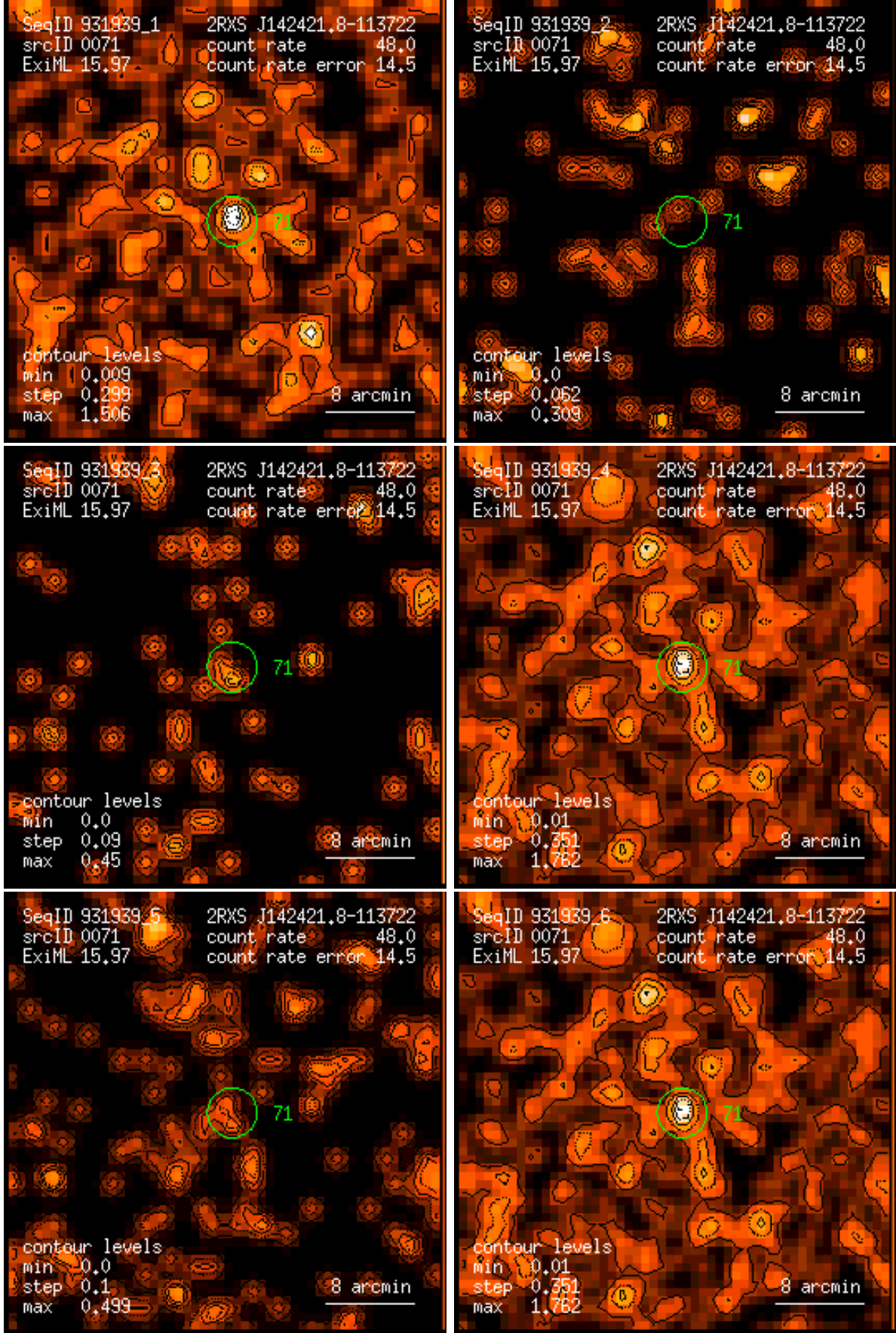
Figure 71: RASS 931939: detection 0071: band rate images, Gaussian filter: (1) PSPC channels 11 – 41, (2) 52 – 90, (3) 91 – 201, (4) 11 – 235, (5) 52 – 201, (6) 11 – 201. Broad band rates in counts/ks. Band rate contour levels in counts/ks/arcmin 2 .
