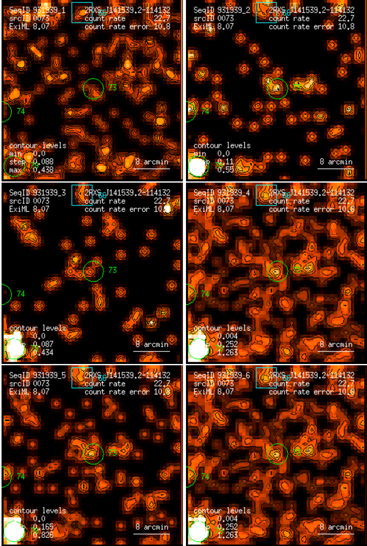
Figure 73: RASS 931939: detection 0073: band rate images, Gaussian filter: (1) PSPC channels 11 – 41, (2) 52 – 90, (3) 91 – 201, (4) 11 – 235, (5) 52 – 201, (6) 11 – 201. Broad band rates in counts/ks. Band rate contour levels in counts/ks/arcmin 2 .
