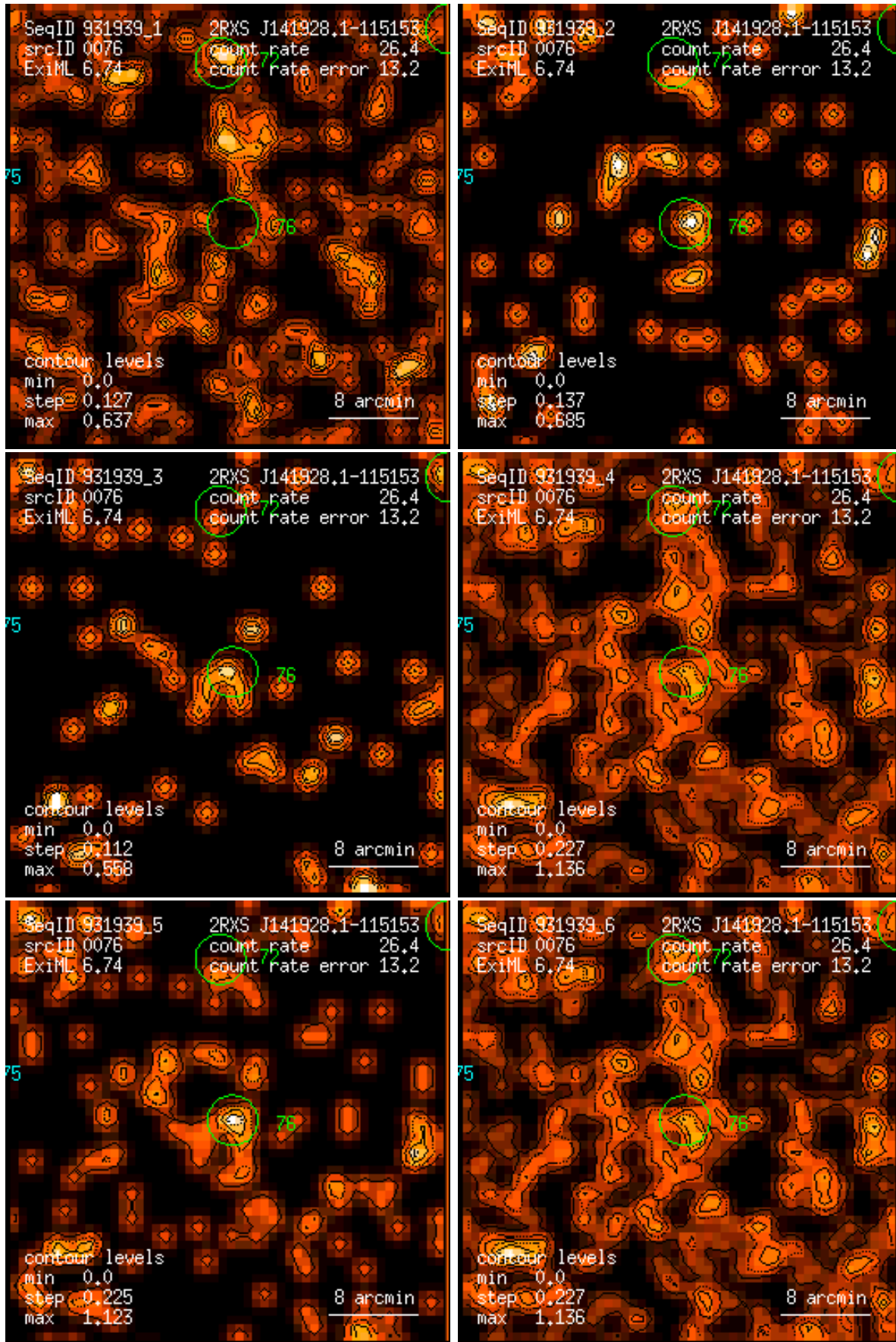
Figure 76: RASS 931939: detection 0076: band rate images, Gaussian filter: (1) PSPC channels 11 – 41, (2) 52 – 90, (3) 91 – 201, (4) 11 – 235, (5) 52 – 201, (6) 11 – 201. Broad band rates in counts/ks. Band rate contour levels in counts/ks/arcmin 2 .
