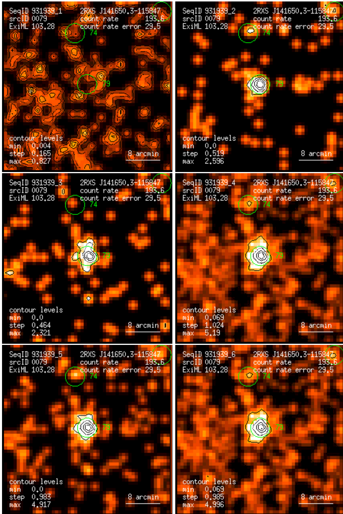
Figure 79: RASS 931939: detection 0079: band rate images, Gaussian filter: (1) PSPC channels 11 – 41, (2) 52 – 90, (3) 91 – 201, (4) 11 – 235, (5) 52 – 201, (6) 11 – 201. Broad band rates in counts/ks. Band rate contour levels in counts/ks/arcmin 2 .
