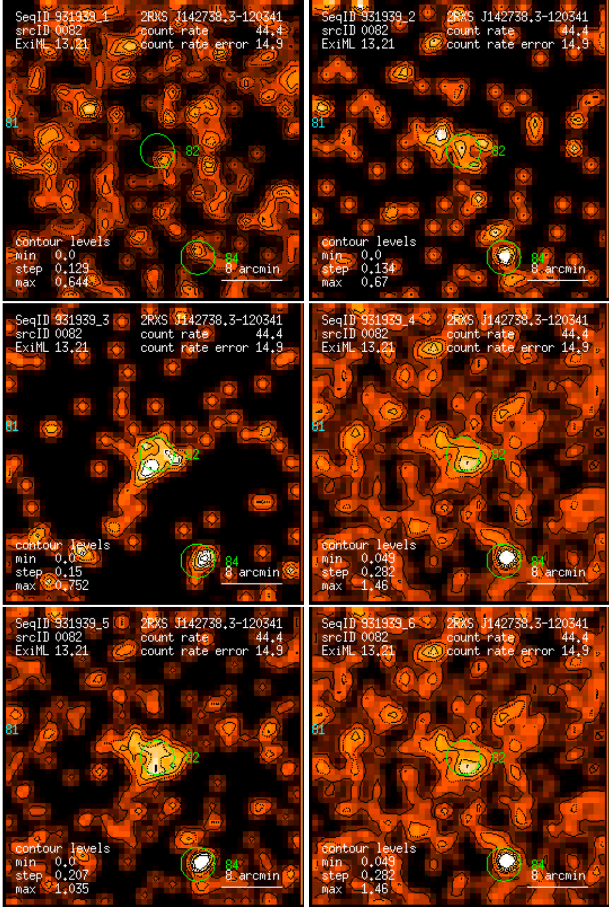
Figure 82: RASS 931939: detection 0082: band rate images, Gaussian filter: (1) PSPC channels 11 – 41, (2) 52 – 90, (3) 91 – 201, (4) 11 – 235, (5) 52 – 201, (6) 11 – 201. Broad band rates in counts/ks. Band rate contour levels in counts/ks/arcmin 2 .
