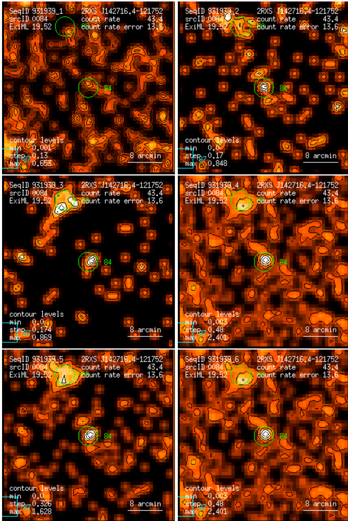
Figure 84: RASS 931939: detection 0084: band rate images, Gaussian filter: (1) PSPC channels 11 – 41, (2) 52 – 90, (3) 91 – 201, (4) 11 – 235, (5) 52 – 201, (6) 11 – 201. Broad band rates in counts/ks. Band rate contour levels in counts/ks/arcmin 2 .
